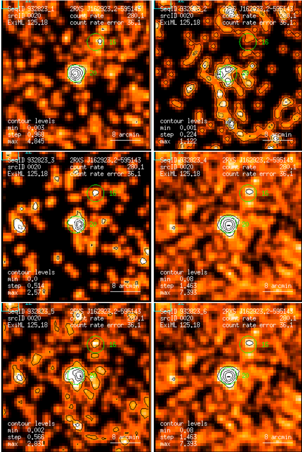
Figure 20: RASS 932823: detection 0020: band rate images, Gaussian filter: (1) PSPC channels 11 – 41, (2) 52 – 90, (3) 91 – 201, (4) 11 – 235, (5) 52 – 201, (6) 11 – 201. Broad band rates in counts/ks. Band rate contour levels in counts/ks/arcmin 2 .
