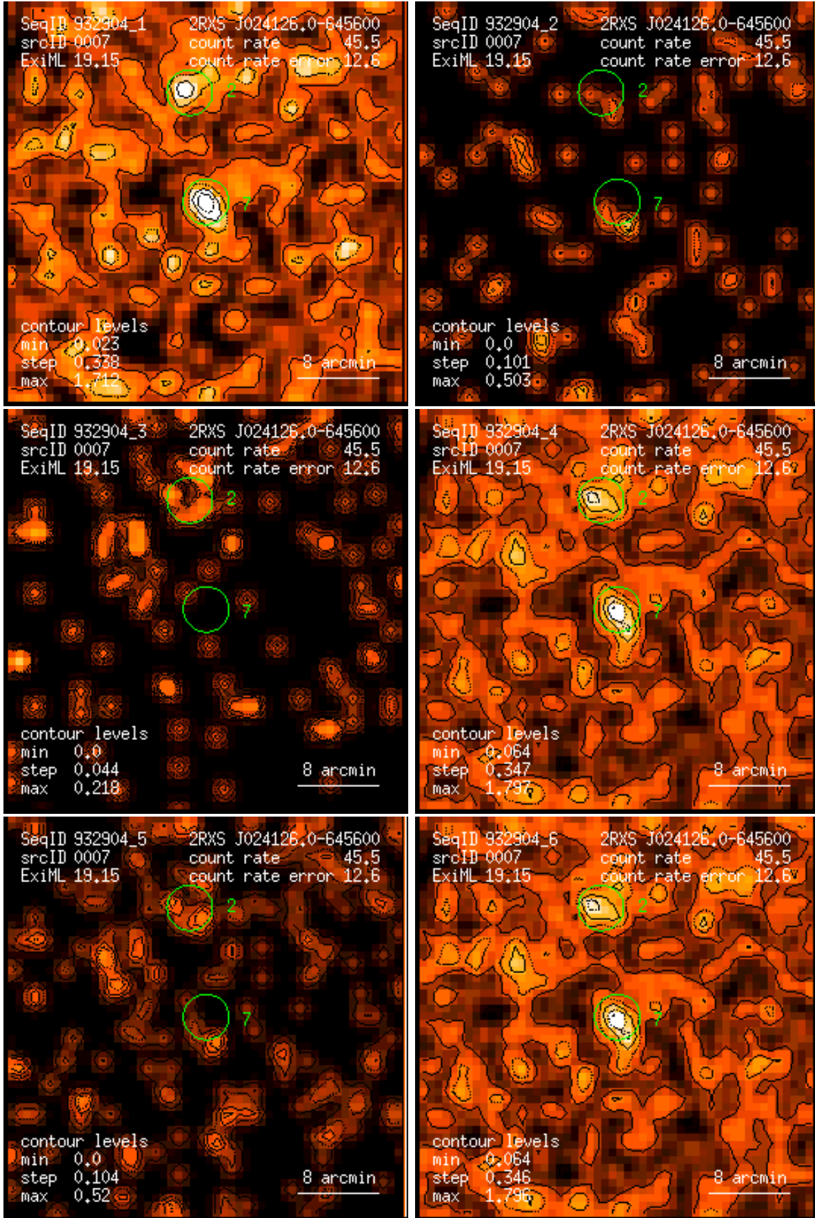
Figure 7: RASS 932904: detection 0007: band rate images, Gaussian filter: (1) PSPC channels 11 – 41, (2) 52 – 90, (3) 91 – 201, (4) 11 – 235, (5) 52 – 201, (6) 11 – 201. Broad band rates in counts/ks. Band rate contour levels in counts/ks/arcmin 2 .
