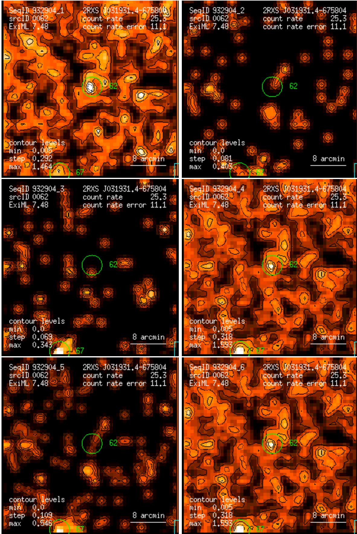
Figure 62: RASS 932904: detection 0062: band rate images, Gaussian filter: (1) PSPC channels 11 – 41, (2) 52 – 90, (3) 91 – 201, (4) 11 – 235, (5) 52 – 201, (6) 11 – 201. Broad band rates in counts/ks. Band rate contour levels in counts/ks/arcmin 2 .
