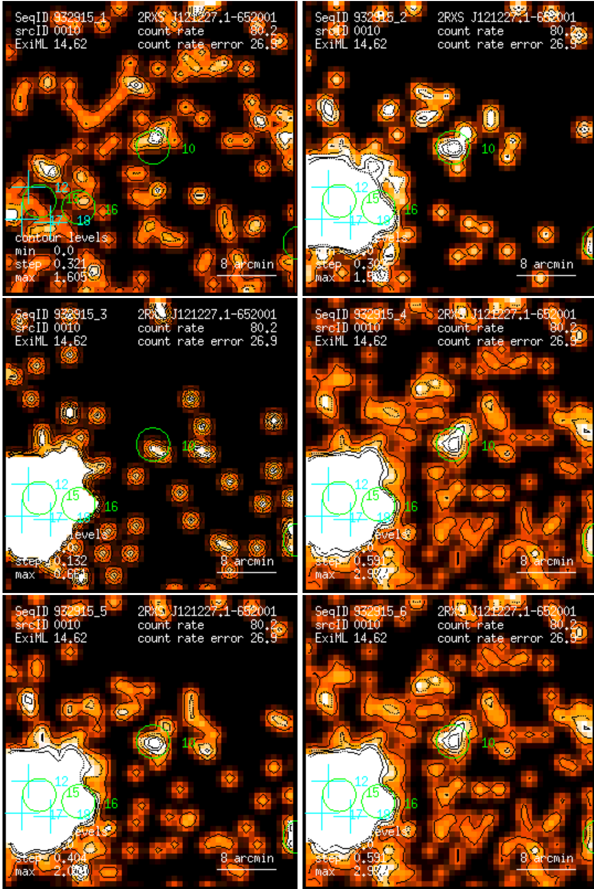
Figure 10: RASS 932915: detection 0010: band rate images, Gaussian filter: (1) PSPC channels 11 – 41, (2) 52 – 90, (3) 91 – 201, (4) 11 – 235, (5) 52 – 201, (6) 11 – 201. Broad band rates in counts/ks. Band rate contour levels in counts/ks/arcmin 2 .
