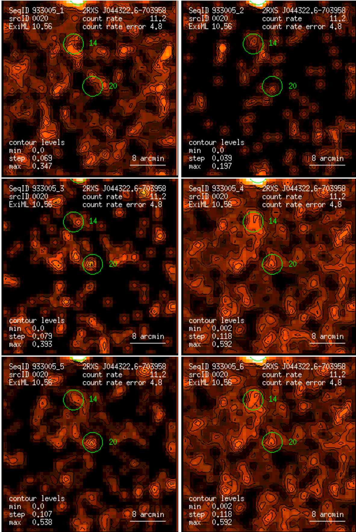
Figure 20: RASS 933005: detection 0020: band rate images, Gaussian filter: (1) PSPC channels 11 – 41, (2) 52 – 90, (3) 91 – 201, (4) 11 – 235, (5) 52 – 201, (6) 11 – 201. Broad band rates in counts/ks. Band rate contour levels in counts/ks/arcmin 2 .
