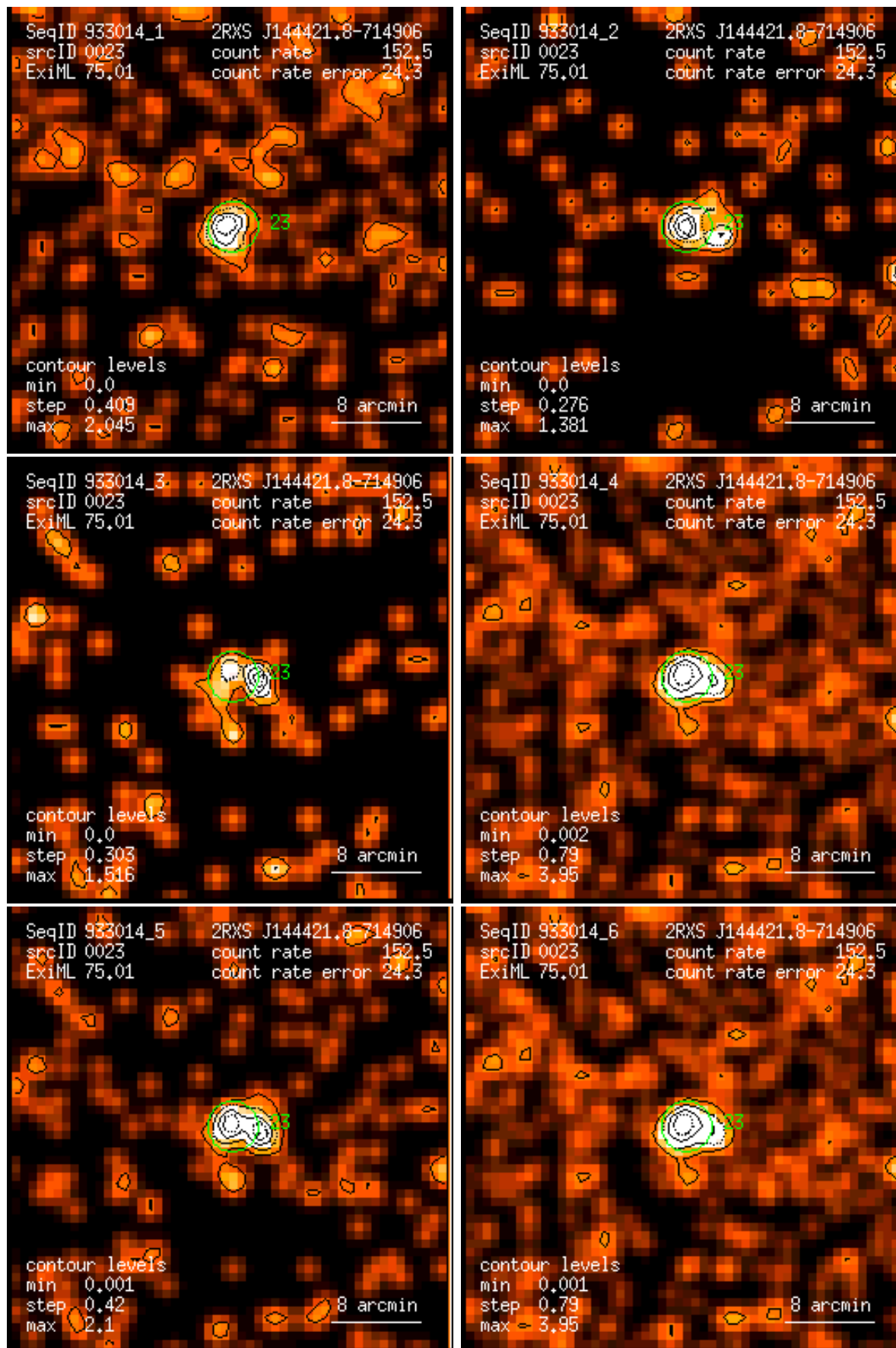
Figure 23: RASS 933014: detection 0023: band rate images, Gaussian filter: (1) PSPC channels 11 – 41, (2) 52 – 90, (3) 91 – 201, (4) 11 – 235, (5) 52 – 201, (6) 11 – 201. Broad band rates in counts/ks. Band rate contour levels in counts/ks/arcmin 2 .
