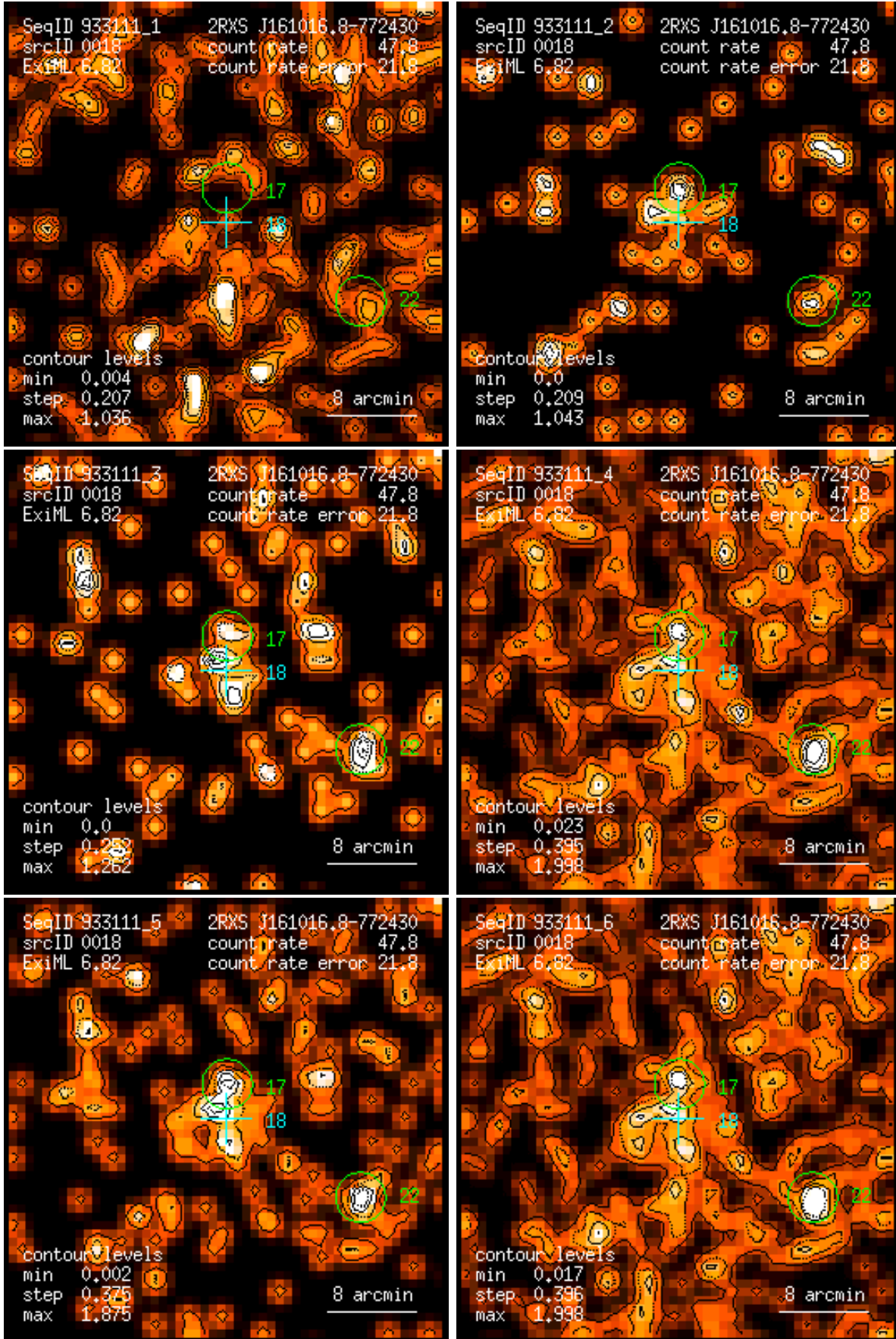
Figure 18: RASS 933111: detection 0018: band rate images, Gaussian filter: (1) PSPC channels 11 – 41, (2) 52 – 90, (3) 91 – 201, (4) 11 – 235, (5) 52 – 201, (6) 11 – 201. Broad band rates in counts/ks. Band rate contour levels in counts/ks/arcmin 2 .
