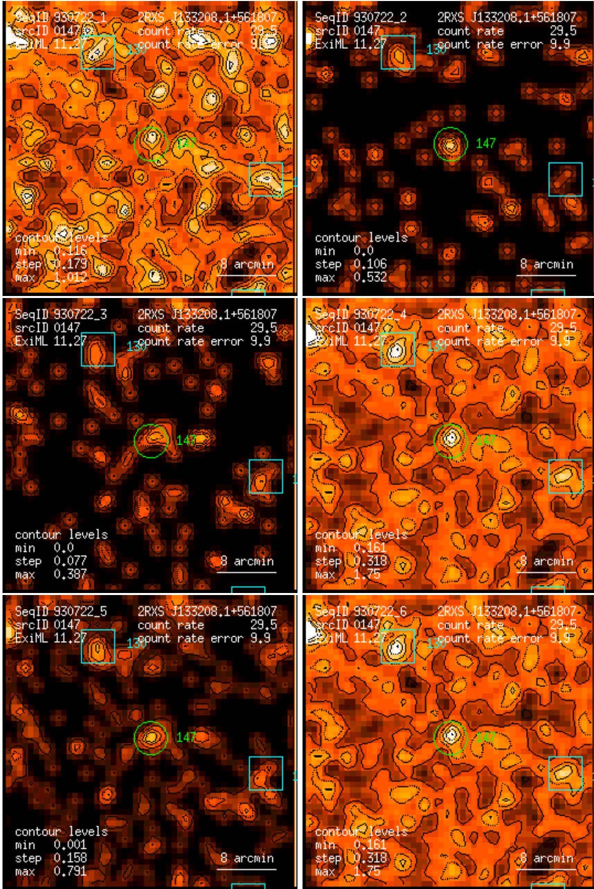
Figure 147: RASS 930722: detection 0147: band rate images, Gaussian filter: (1) PSPC channels 11 – 41, (2) 52 – 90, (3) 91 – 201, (4) 11 – 235, (5) 52 – 201, (6) 11 – 201. Broad band rates in counts/ks. Band rate contour levels in counts/ks/arcmin 2 .
