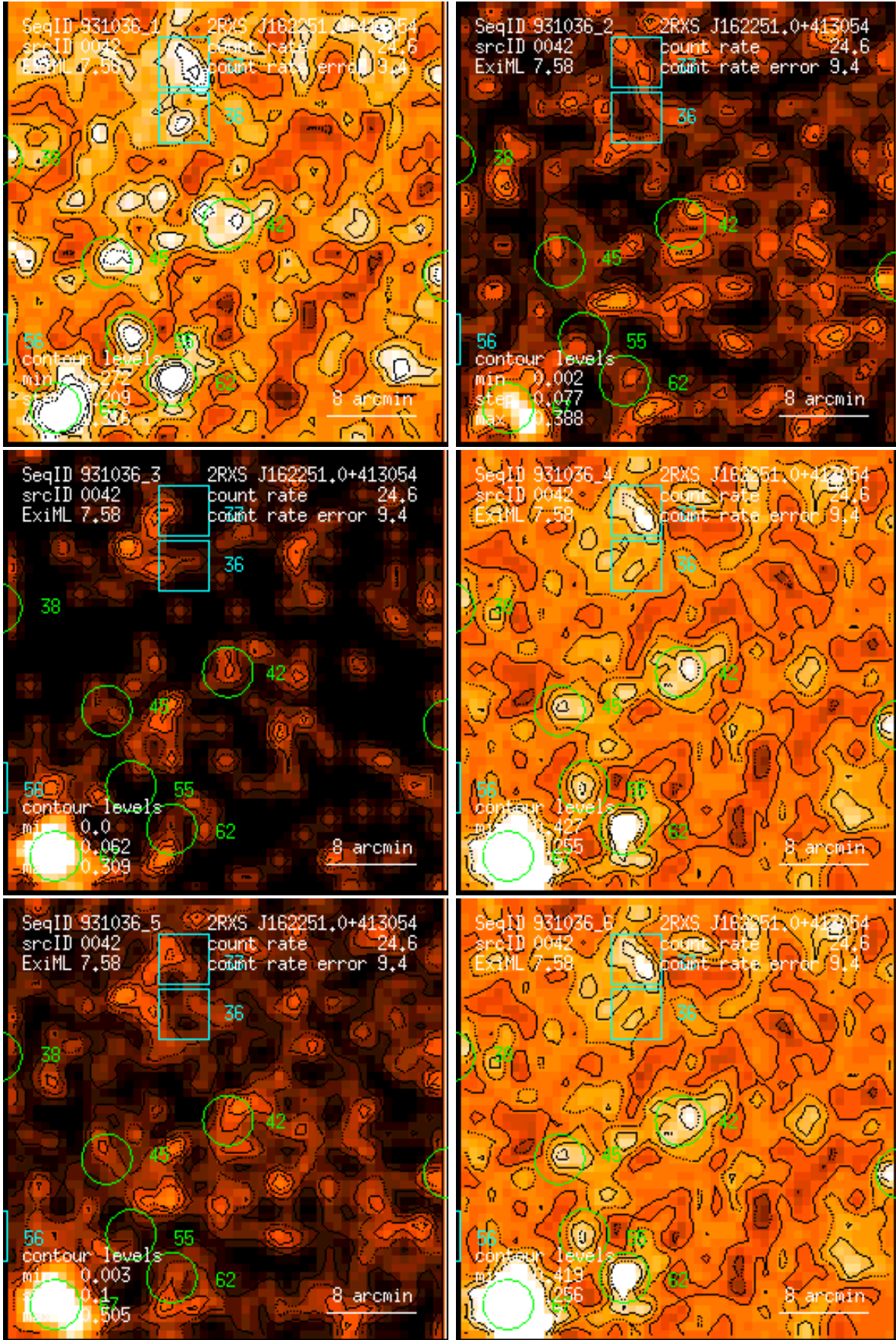
Figure 42: RASS 931036: detection 0042: band rate images, Gaussian filter: (1) PSPC channels 11 – 41, (2) 52 – 90, (3) 91 – 201, (4) 11 – 235, (5) 52 – 201, (6) 11 – 201. Broad band rates in counts/ks. Band rate contour levels in counts/ks/arcmin 2 .
