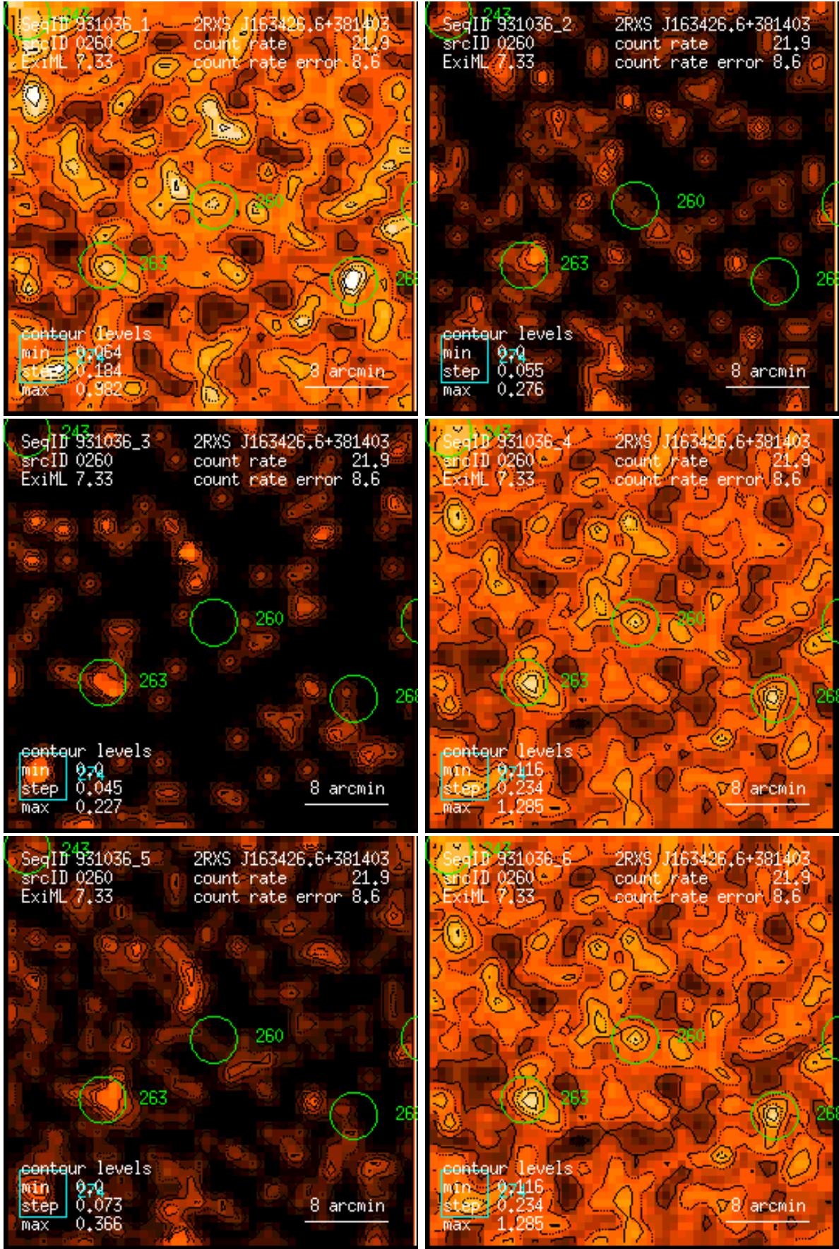
Figure 260: RASS 931036: detection 0260: band rate images, Gaussian filter: (1) PSPC channels 11 – 41, (2) 52 – 90, (3) 91 – 201, (4) 11 – 235, (5) 52 – 201, (6) 11 – 201. Broad band rates in counts/ks. Band rate contour levels in counts/ks/arcmin 2 .
