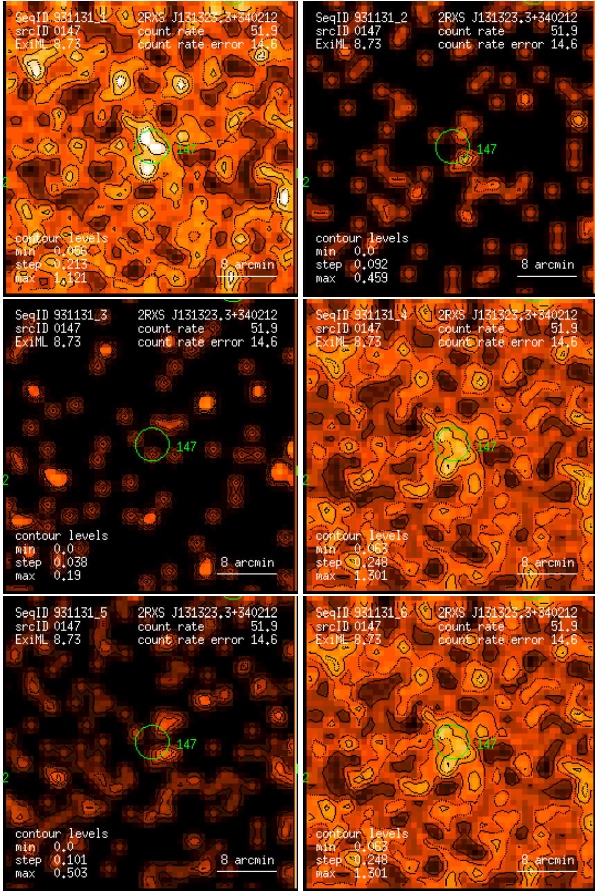
Figure 147: RASS 931131: detection 0147: band rate images, Gaussian filter: (1) PSPC channels 11 – 41, (2) 52 – 90, (3) 91 – 201, (4) 11 – 235, (5) 52 – 201, (6) 11 – 201. Broad band rates in counts/ks. Band rate contour levels in counts/ks/arcmin 2 .
