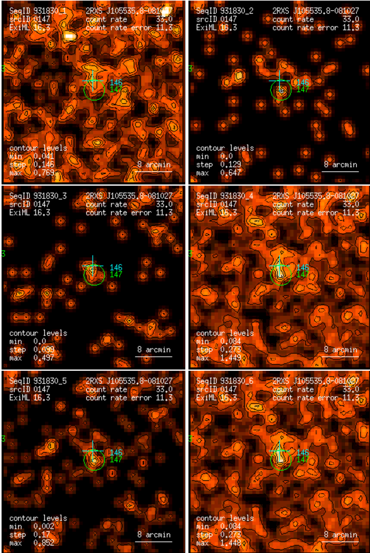
Figure 147: RASS 931830: detection 0147: band rate images, Gaussian filter: (1) PSPC channels 11 – 41, (2) 52 – 90, (3) 91 – 201, (4) 11 – 235, (5) 52 – 201, (6) 11 – 201. Broad band rates in counts/ks. Band rate contour levels in counts/ks/arcmin 2 .
