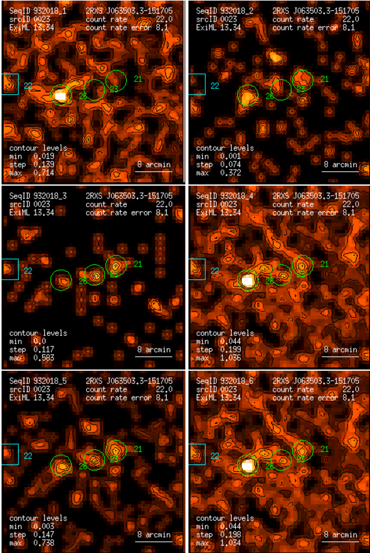
Figure 23: RASS 932018: detection 0023: band rate images, Gaussian filter: (1) PSPC channels 11 – 41, (2) 52 – 90, (3) 91 – 201, (4) 11 – 235, (5) 52 – 201, (6) 11 – 201. Broad band rates in counts/ks. Band rate contour levels in counts/ks/arcmin 2 .
