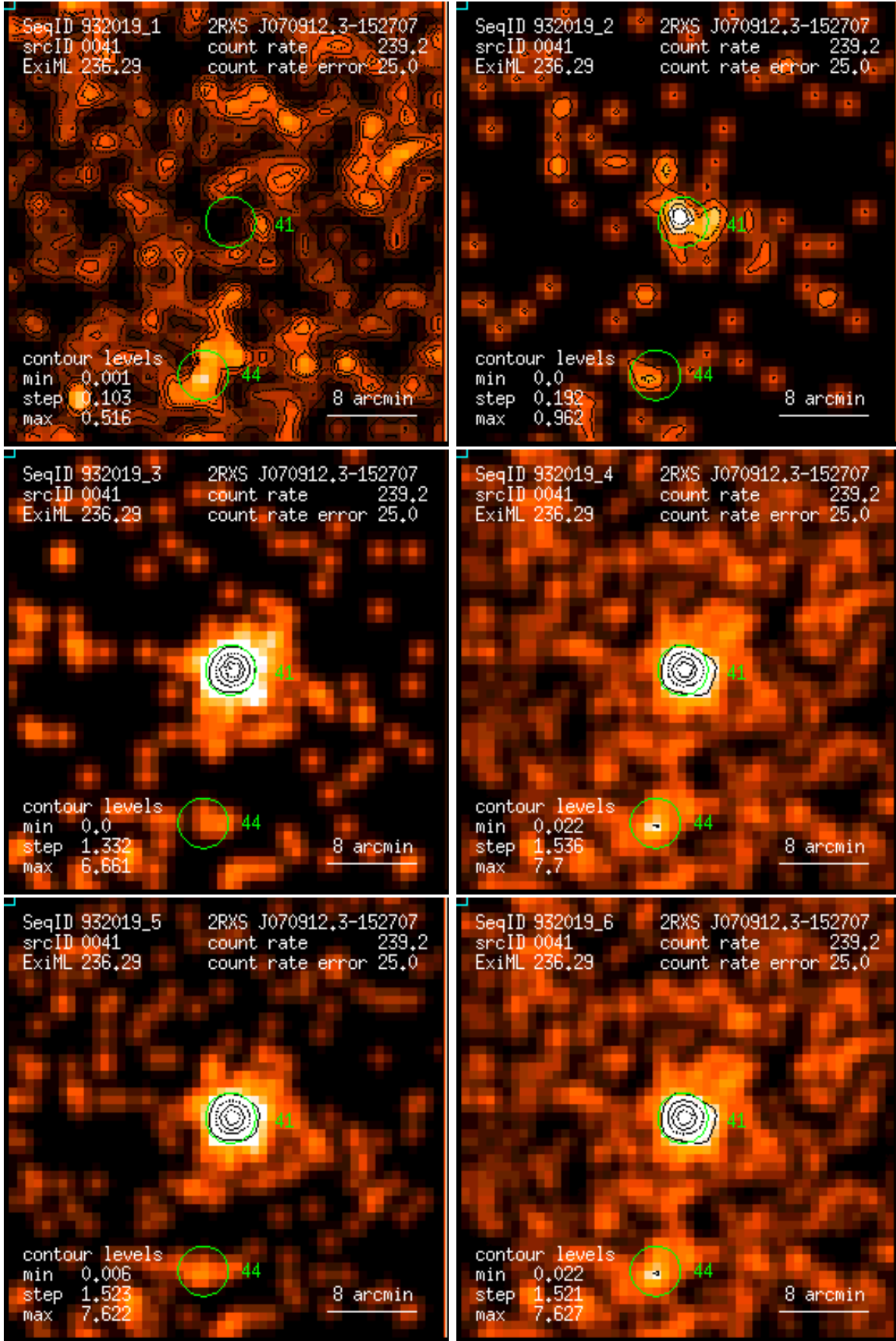
Figure 41: RASS 932019: detection 0041: band rate images, Gaussian filter: (1) PSPC channels 11 – 41, (2) 52 – 90, (3) 91 – 201, (4) 11 – 235, (5) 52 – 201, (6) 11 – 201. Broad band rates in counts/ks. Band rate contour levels in counts/ks/arcmin 2 .
