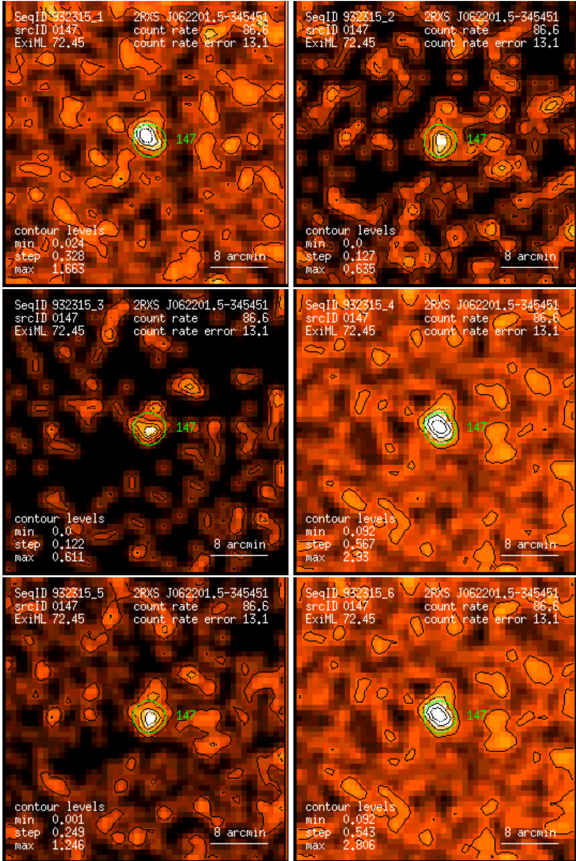
Figure 147: RASS 932315: detection 0147: band rate images, Gaussian filter: (1) PSPC channels 11 – 41, (2) 52 – 90, (3) 91 – 201, (4) 11 – 235, (5) 52 – 201, (6) 11 – 201. Broad band rates in counts/ks. Band rate contour levels in counts/ks/arcmin 2 .
