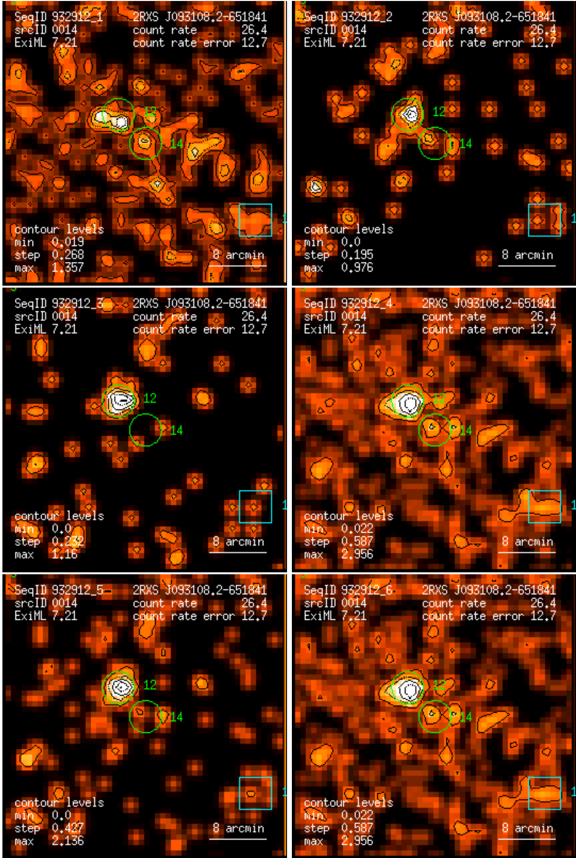
Figure 14: RASS 932912: detection 0014: band rate images, Gaussian filter: (1) PSPC channels 11 – 41, (2) 52 – 90, (3) 91 – 201, (4) 11 – 235, (5) 52 – 201, (6) 11 – 201. Broad band rates in counts/ks. Band rate contour levels in counts/ks/arcmin 2 .
