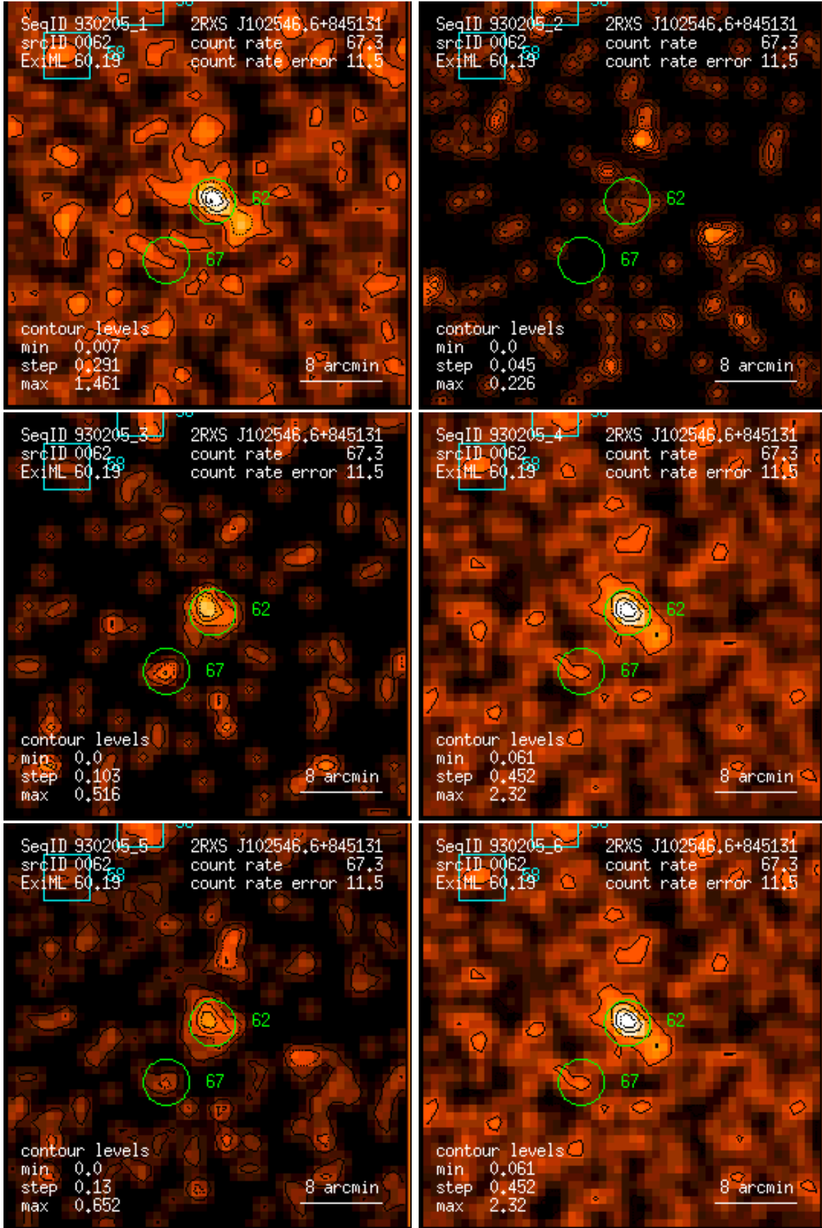
Figure 62: RASS 930205: detection 0062: band rate images, Gaussian filter: (1) PSPC channels 11 – 41, (2) 52 – 90, (3) 91 – 201, (4) 11 – 235, (5) 52 – 201, (6) 11 – 201. Broad band rates in counts/ks. Band rate contour levels in counts/ks/arcmin 2 .
