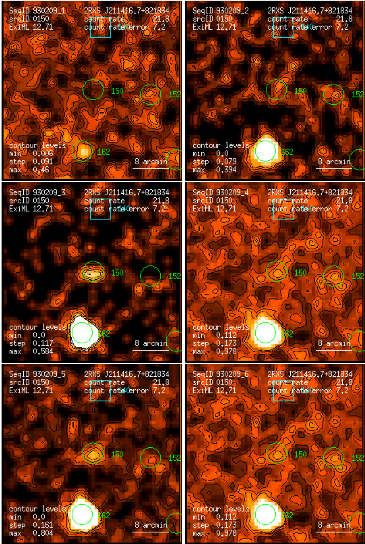
Figure 150: RASS 930209: detection 0150: band rate images, Gaussian filter: (1) PSPC channels 11 – 41, (2) 52 – 90, (3) 91 – 201, (4) 11 – 235, (5) 52 – 201, (6) 11 – 201. Broad band rates in counts/ks. Band rate contour levels in counts/ks/arcmin 2 .
