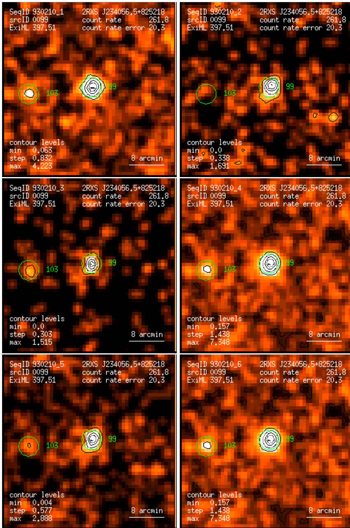
Figure 99: RASS 930210: detection 0099: band rate images, Gaussian filter: (1) PSPC channels 11 – 41, (2) 52 – 90, (3) 91 – 201, (4) 11 – 235, (5) 52 – 201, (6) 11 – 201. Broad band rates in counts/ks. Band rate contour levels in counts/ks/arcmin 2 .
