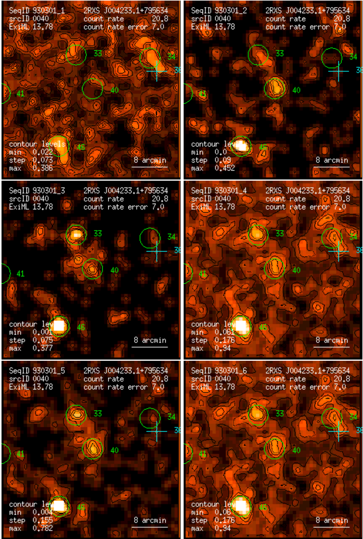
Figure 40: RASS 930301: detection 0040: band rate images, Gaussian filter: (1) PSPC channels 11 – 41, (2) 52 – 90, (3) 91 – 201, (4) 11 – 235, (5) 52 – 201, (6) 11 – 201. Broad band rates in counts/ks. Band rate contour levels in counts/ks/arcmin 2 .
