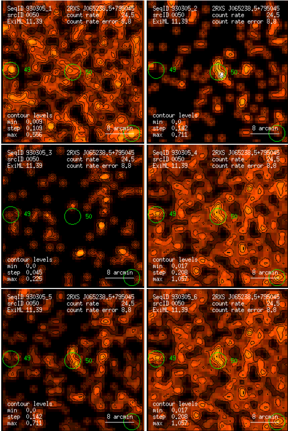
Figure 50: RASS 930305: detection 0050: band rate images, Gaussian filter: (1) PSPC channels 11 – 41, (2) 52 – 90, (3) 91 – 201, (4) 11 – 235, (5) 52 – 201, (6) 11 – 201. Broad band rates in counts/ks. Band rate contour levels in counts/ks/arcmin 2 .
