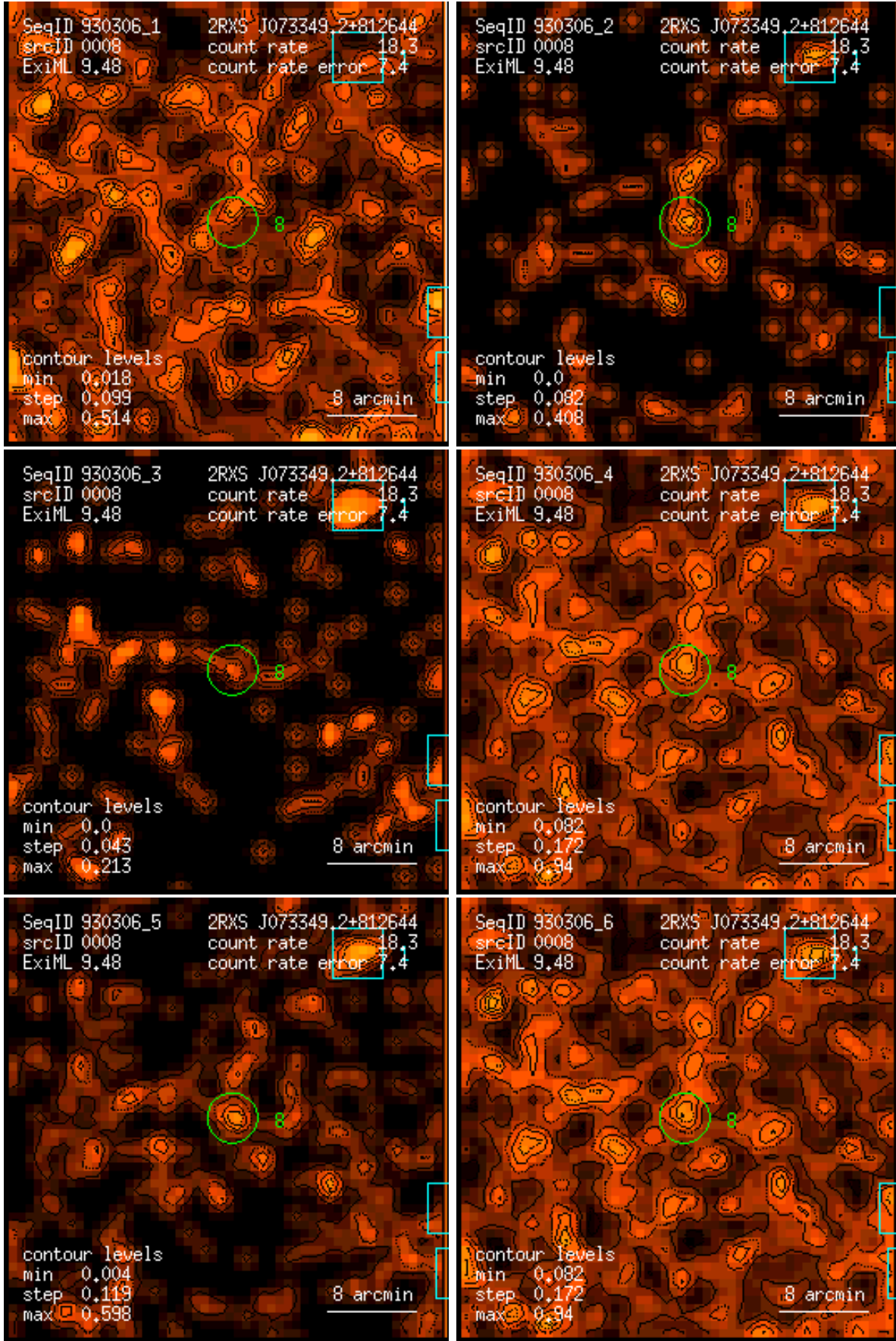
Figure 8: RASS 930306: detection 0008: band rate images, Gaussian filter: (1) PSPC channels 11 – 41, (2) 52 – 90, (3) 91 – 201, (4) 11 – 235, (5) 52 – 201, (6) 11 – 201. Broad band rates in counts/ks. Band rate contour levels in counts/ks/arcmin 2 .
