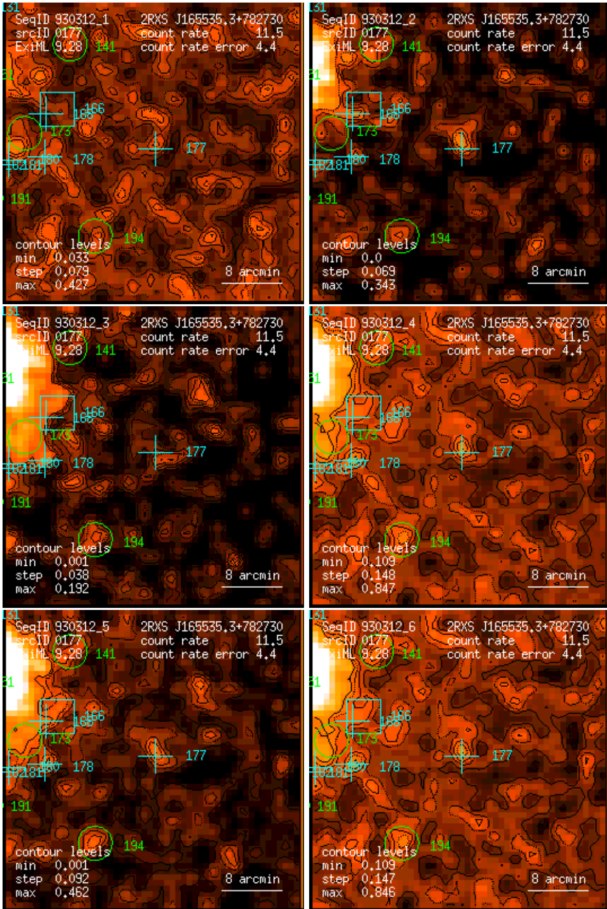
Figure 177: RASS 930312: detection 0177: band rate images, Gaussian filter: (1) PSPC channels 11 – 41, (2) 52 – 90, (3) 91 – 201, (4) 11 – 235, (5) 52 – 201, (6) 11 – 201. Broad band rates in counts/ks. Band rate contour levels in counts/ks/arcmin 2 .
