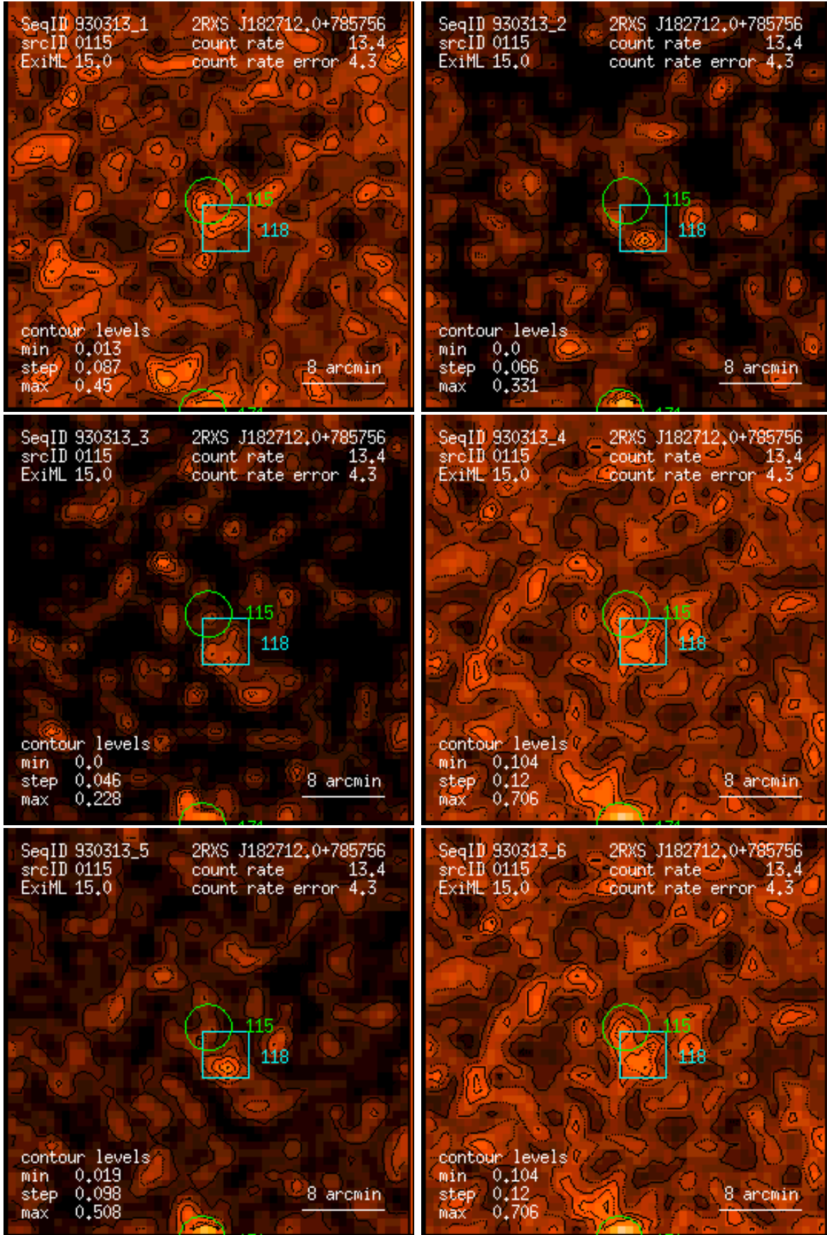
Figure 115: RASS 930313: detection 0115: band rate images, Gaussian filter: (1) PSPC channels 11 – 41, (2) 52 – 90, (3) 91 – 201, (4) 11 – 235, (5) 52 – 201, (6) 11 – 201. Broad band rates in counts/ks. Band rate contour levels in counts/ks/arcmin 2 .
