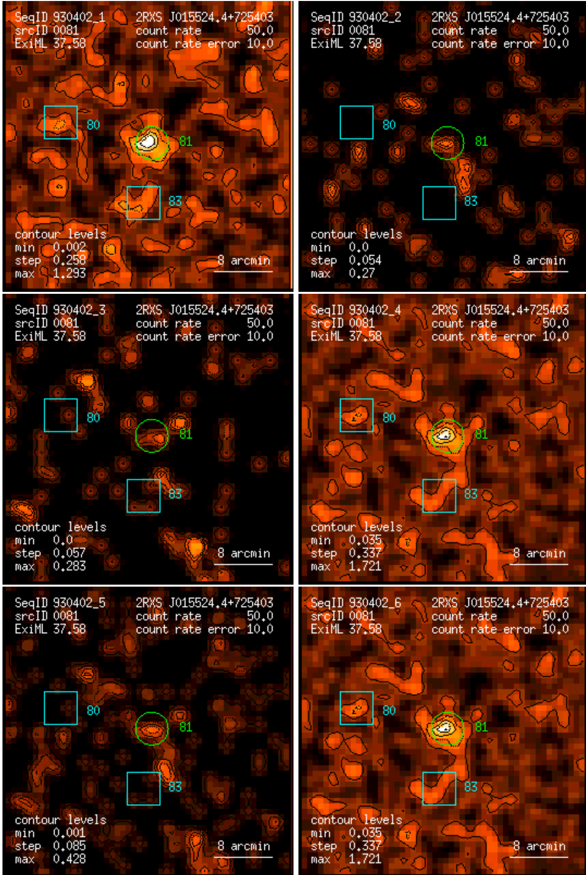
Figure 81: RASS 930402: detection 0081: band rate images, Gaussian filter: (1) PSPC channels 11 – 41, (2) 52 – 90, (3) 91 – 201, (4) 11 – 235, (5) 52 – 201, (6) 11 – 201. Broad band rates in counts/ks. Band rate contour levels in counts/ks/arcmin 2 .
