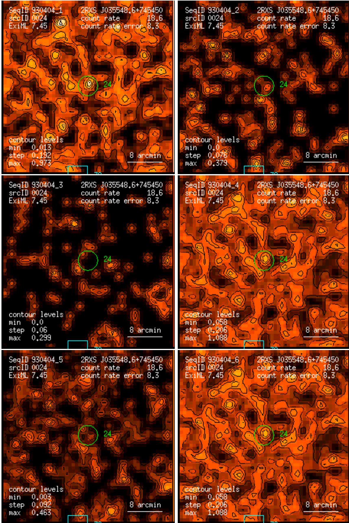
Figure 24: RASS 930404: detection 0024: band rate images, Gaussian filter: (1) PSPC channels 11 – 41, (2) 52 – 90, (3) 91 – 201, (4) 11 – 235, (5) 52 – 201, (6) 11 – 201. Broad band rates in counts/ks. Band rate contour levels in counts/ks/arcmin 2 .
