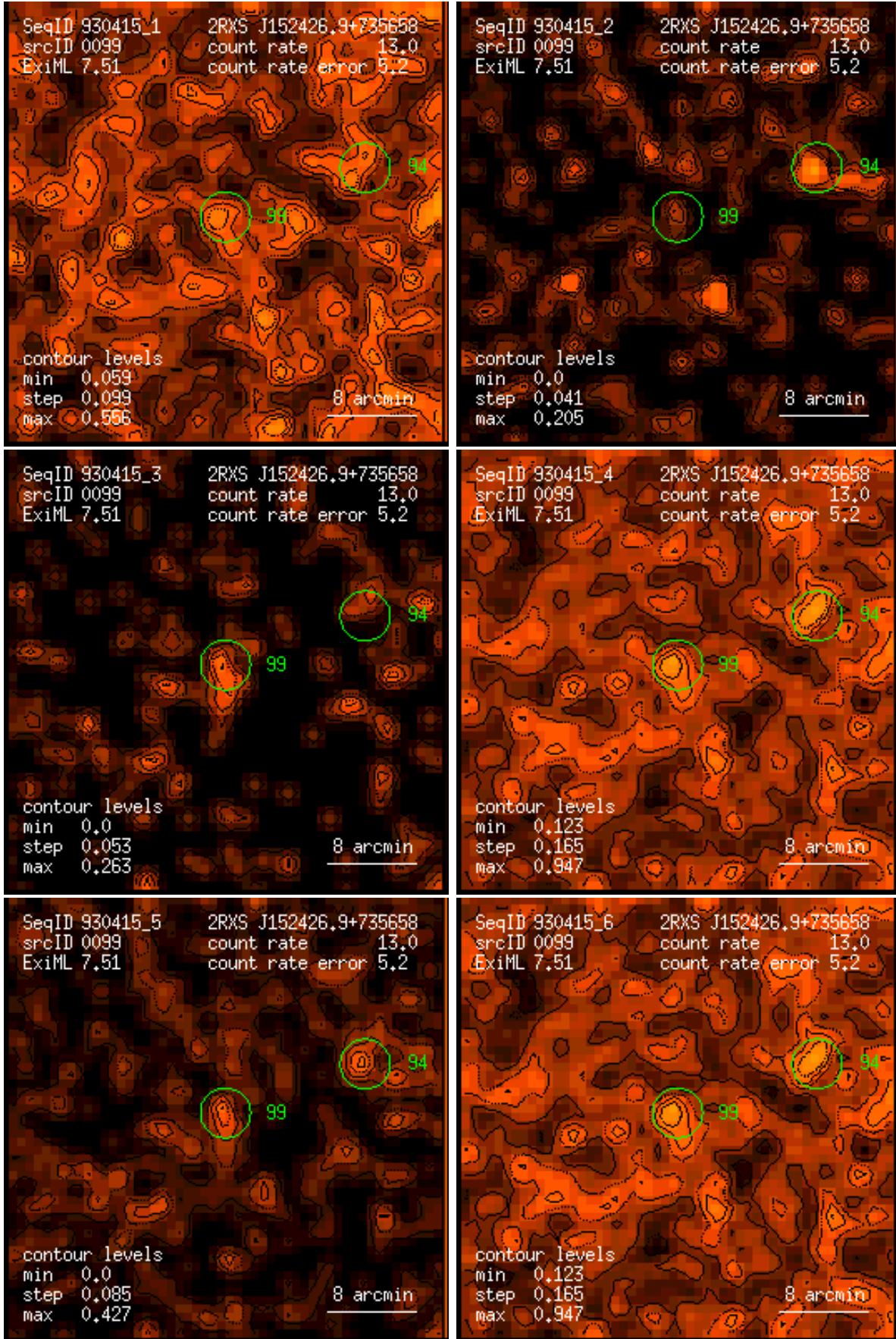
Figure 99: RASS 930415: detection 0099: band rate images, Gaussian filter: (1) PSPC channels 11 – 41, (2) 52 – 90, (3) 91 – 201, (4) 11 – 235, (5) 52 – 201, (6) 11 – 201. Broad band rates in counts/ks. Band rate contour levels in counts/ks/arcmin 2 .
