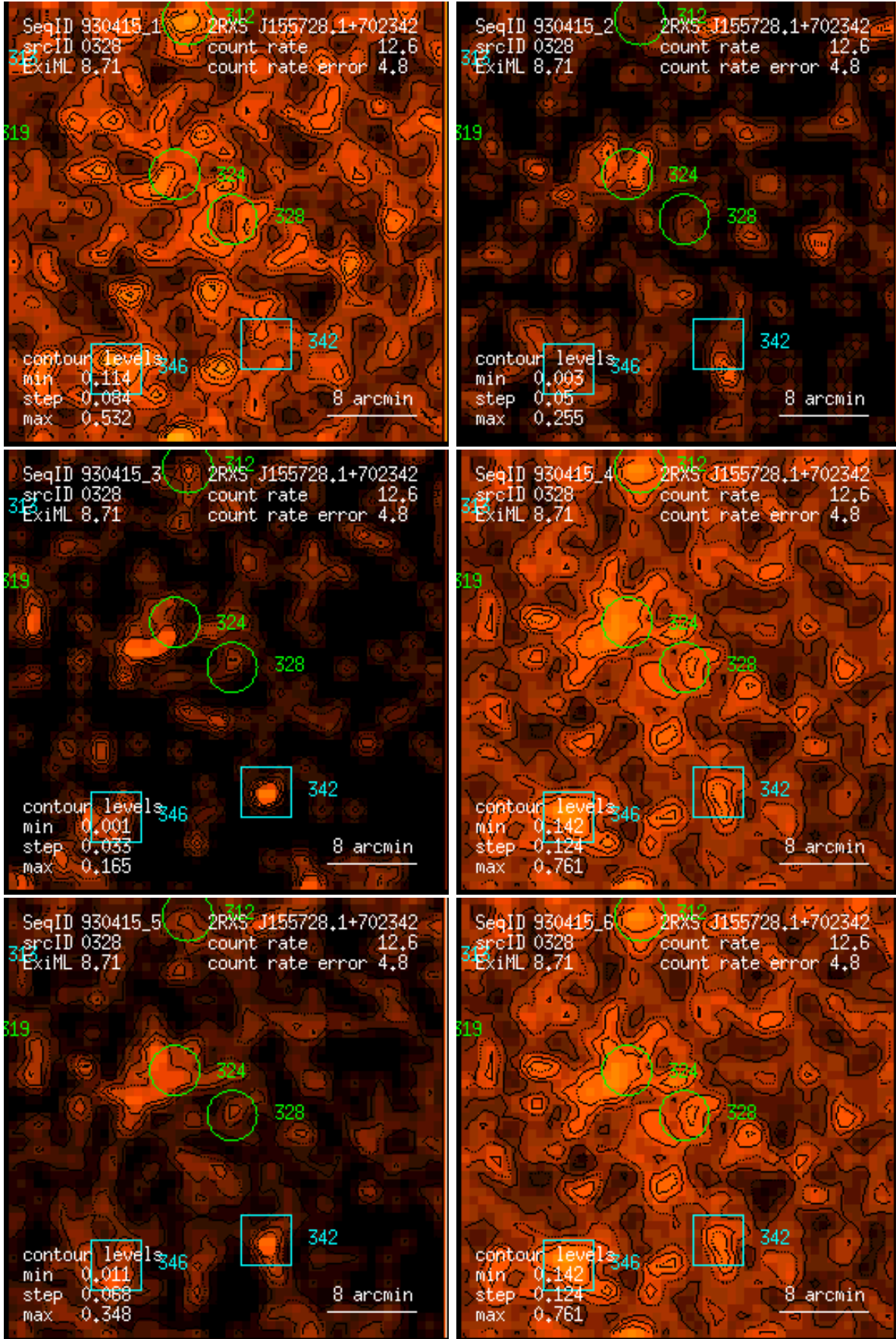
Figure 328: RASS 930415: detection 0328: band rate images, Gaussian filter: (1) PSPC channels 11 – 41, (2) 52 – 90, (3) 91 – 201, (4) 11 – 235, (5) 52 – 201, (6) 11 – 201. Broad band rates in counts/ks. Band rate contour levels in counts/ks/arcmin 2 .
