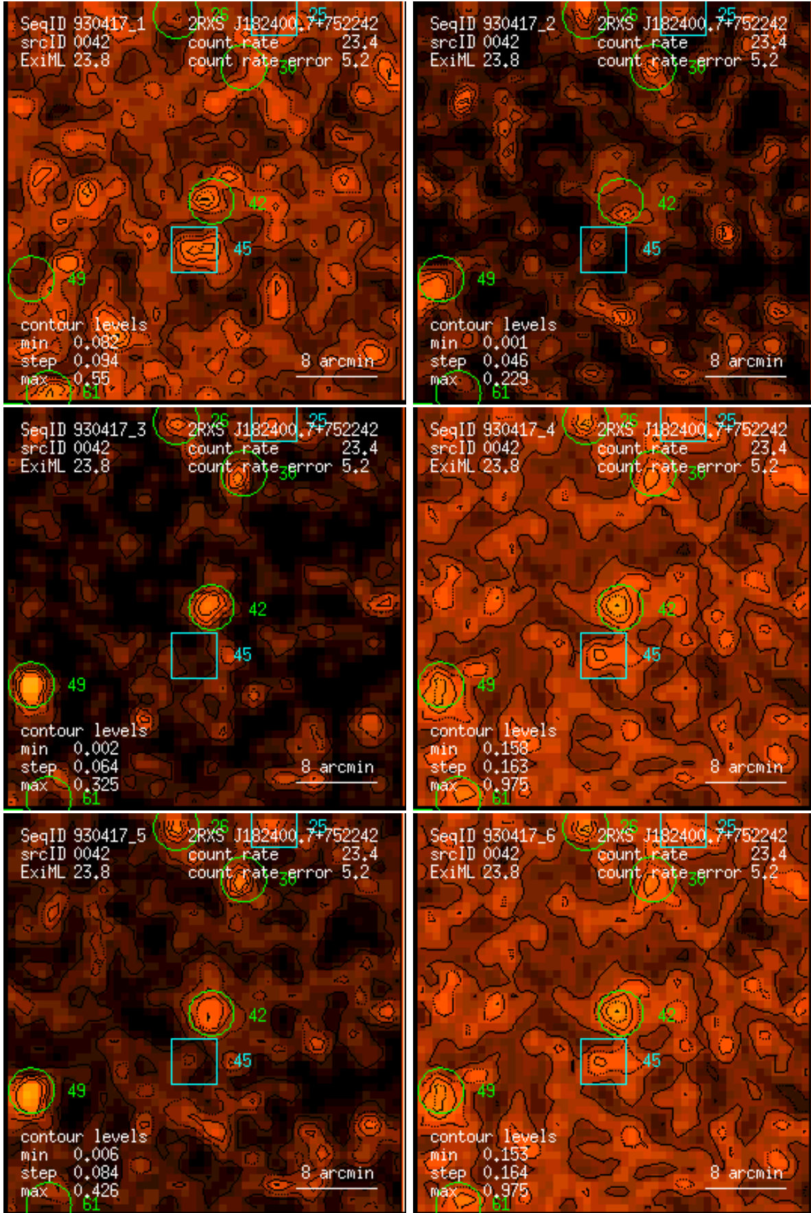
Figure 42: RASS 930417: detection 0042: band rate images, Gaussian filter: (1) PSPC channels 11 – 41, (2) 52 – 90, (3) 91 – 201, (4) 11 – 235, (5) 52 – 201, (6) 11 – 201. Broad band rates in counts/ks. Band rate contour levels in counts/ks/arcmin 2 .
