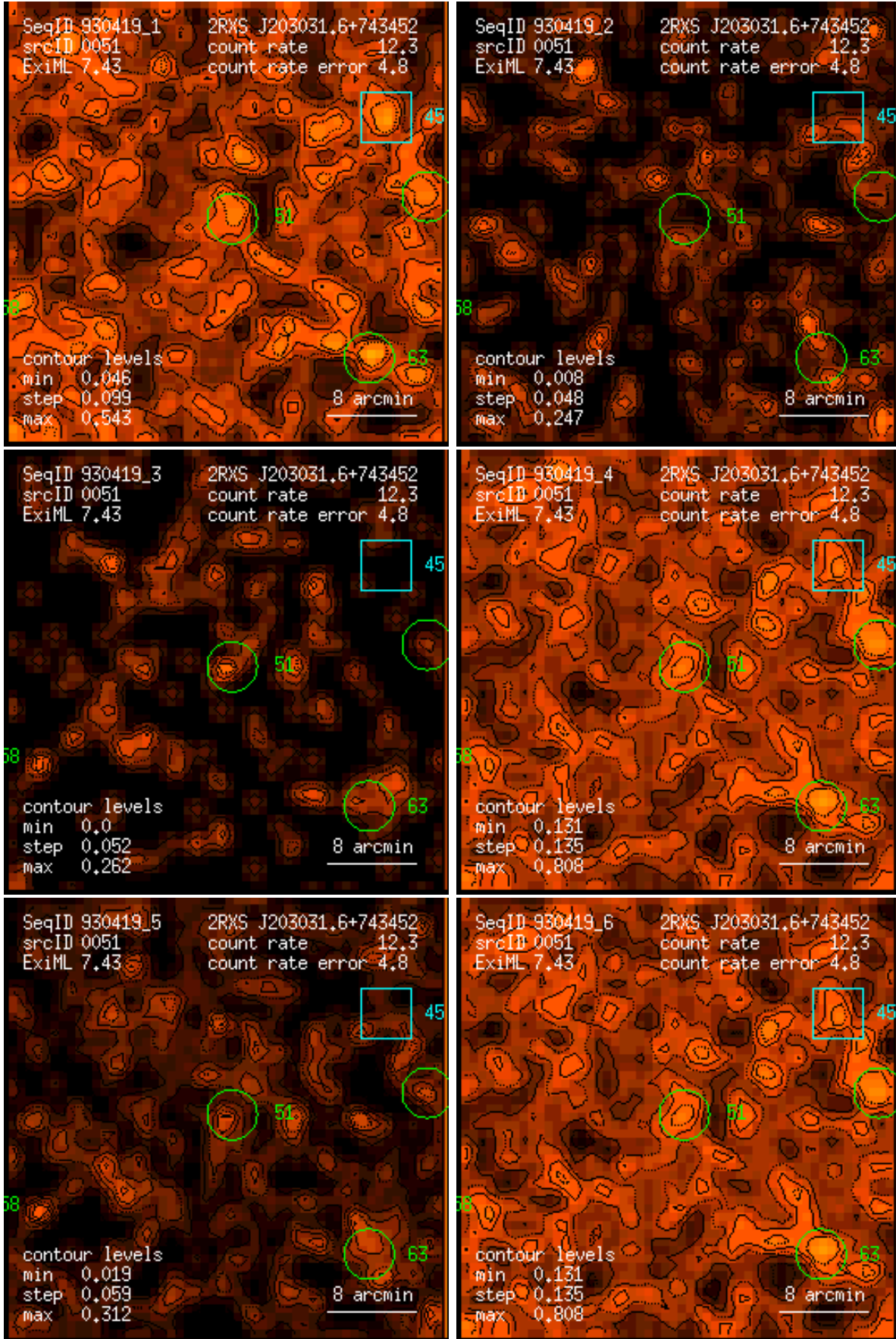
Figure 51: RASS 930419: detection 0051: band rate images, Gaussian filter: (1) PSPC channels 11 – 41, (2) 52 – 90, (3) 91 – 201, (4) 11 – 235, (5) 52 – 201, (6) 11 – 201. Broad band rates in counts/ks. Band rate contour levels in counts/ks/arcmin 2 .
