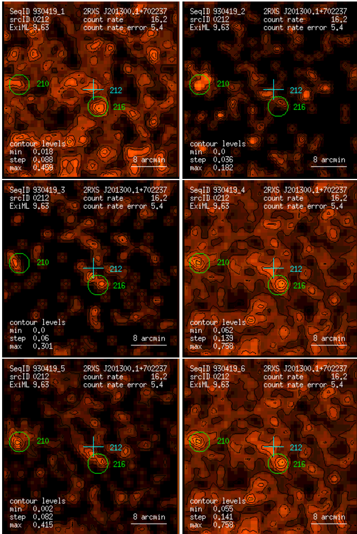
Figure 212: RASS 930419: detection 0212: band rate images, Gaussian filter: (1) PSPC channels 11 – 41, (2) 52 – 90, (3) 91 – 201, (4) 11 – 235, (5) 52 – 201, (6) 11 – 201. Broad band rates in counts/ks. Band rate contour levels in counts/ks/arcmin 2 .
