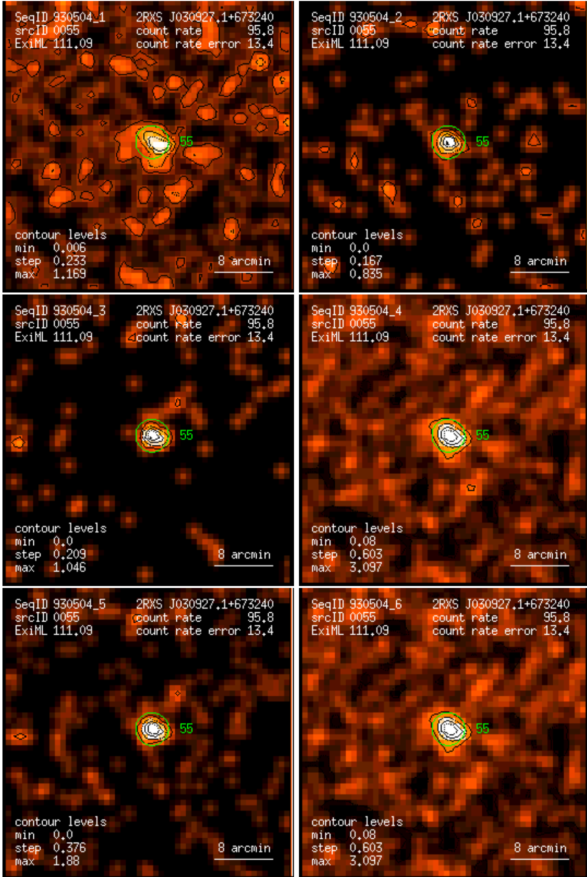
Figure 55: RASS 930504: detection 0055: band rate images, Gaussian filter: (1) PSPC channels 11 – 41, (2) 52 – 90, (3) 91 – 201, (4) 11 – 235, (5) 52 – 201, (6) 11 – 201. Broad band rates in counts/ks. Band rate contour levels in counts/ks/arcmin 2 .
