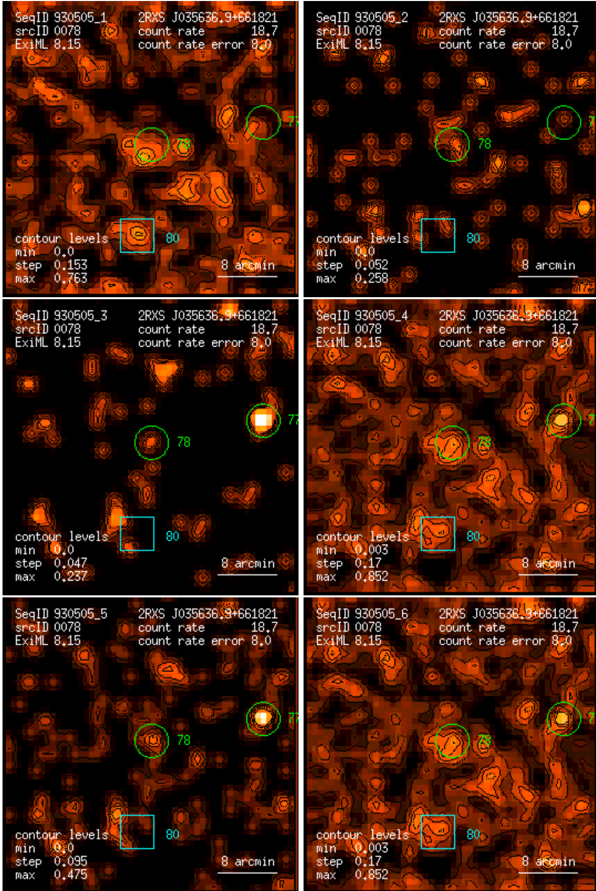
Figure 78: RASS 930505: detection 0078: band rate images, Gaussian filter: (1) PSPC channels 11 – 41, (2) 52 – 90, (3) 91 – 201, (4) 11 – 235, (5) 52 – 201, (6) 11 – 201. Broad band rates in counts/ks. Band rate contour levels in counts/ks/arcmin 2 .
