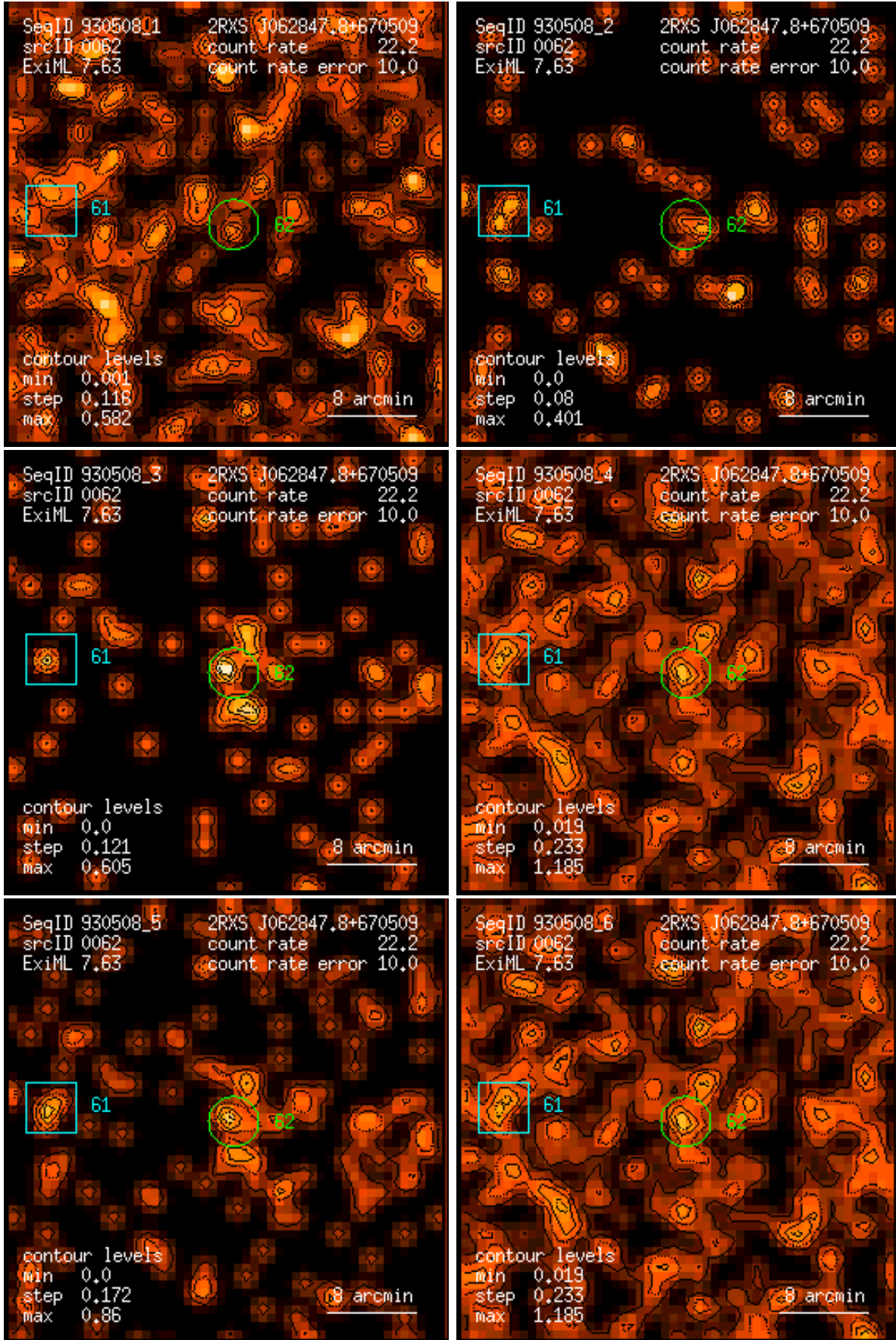
Figure 62: RASS 930508: detection 0062: band rate images, Gaussian filter: (1) PSPC channels 11 – 41, (2) 52 – 90, (3) 91 – 201, (4) 11 – 235, (5) 52 – 201, (6) 11 – 201. Broad band rates in counts/ks. Band rate contour levels in counts/ks/arcmin 2 .
