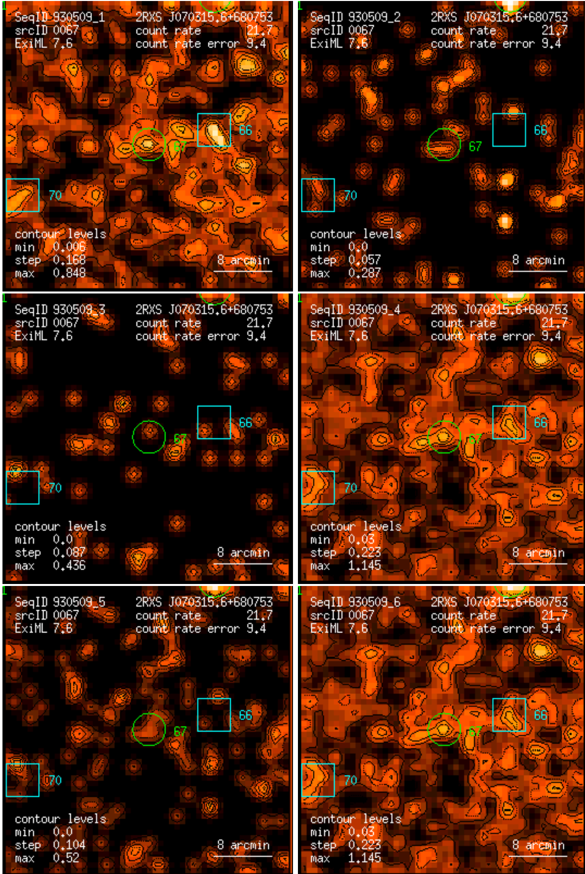
Figure 67: RASS 930509: detection 0067: band rate images, Gaussian filter: (1) PSPC channels 11 – 41, (2) 52 – 90, (3) 91 – 201, (4) 11 – 235, (5) 52 – 201, (6) 11 – 201. Broad band rates in counts/ks. Band rate contour levels in counts/ks/arcmin 2 .
