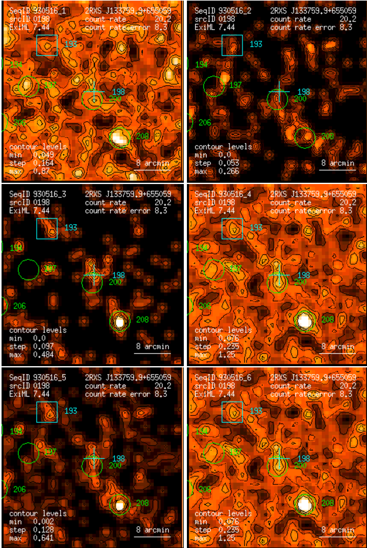
Figure 198: RASS 930516: detection 0198: band rate images, Gaussian filter: (1) PSPC channels 11 – 41, (2) 52 – 90, (3) 91 – 201, (4) 11 – 235, (5) 52 – 201, (6) 11 – 201. Broad band rates in counts/ks. Band rate contour levels in counts/ks/arcmin 2 .
