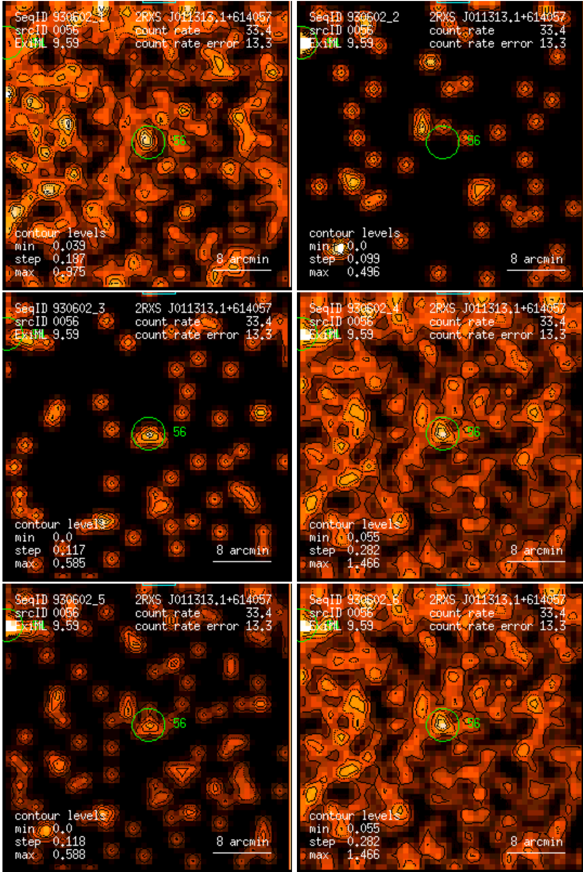
Figure 56: RASS 930602: detection 0056: band rate images, Gaussian filter: (1) PSPC channels 11 – 41, (2) 52 – 90, (3) 91 – 201, (4) 11 – 235, (5) 52 – 201, (6) 11 – 201. Broad band rates in counts/ks. Band rate contour levels in counts/ks/arcmin 2 .
