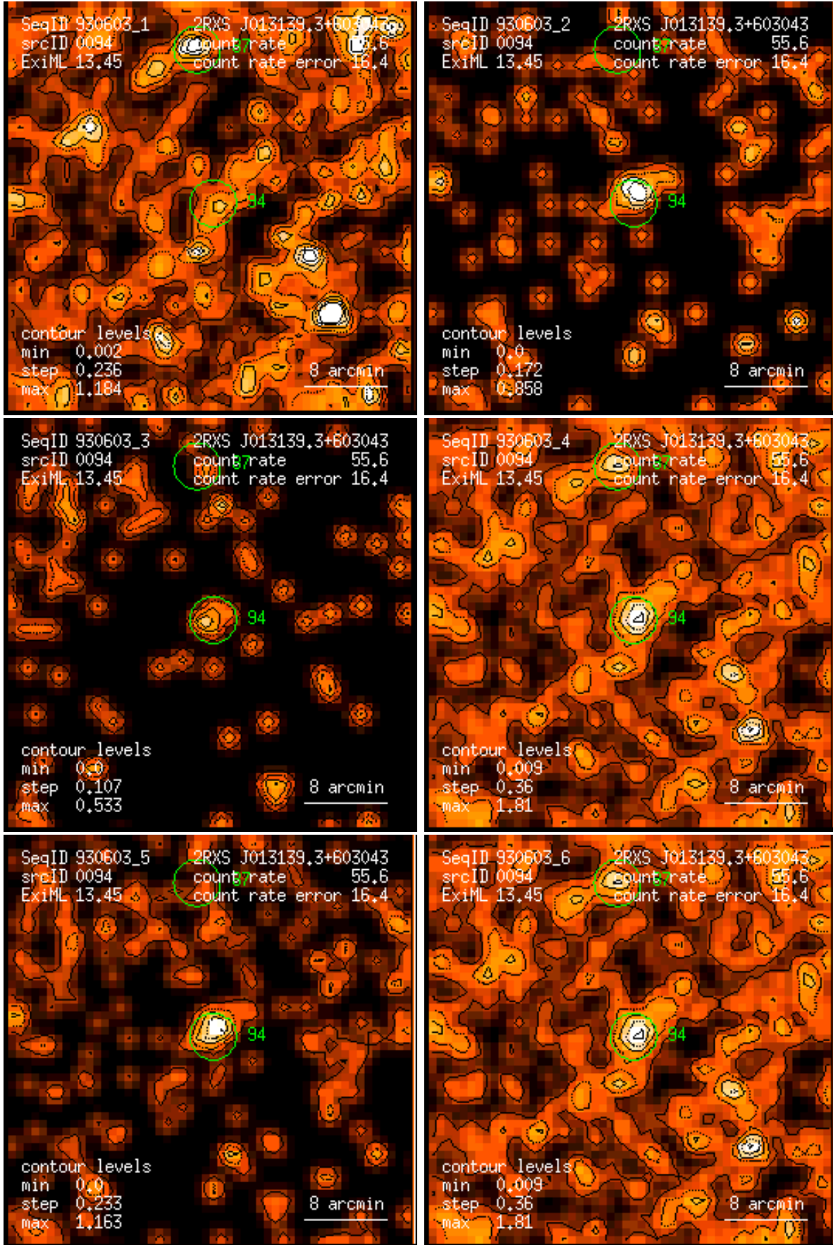
Figure 94: RASS 930603: detection 0094: band rate images, Gaussian filter: (1) PSPC channels 11 – 41, (2) 52 – 90, (3) 91 – 201, (4) 11 – 235, (5) 52 – 201, (6) 11 – 201. Broad band rates in counts/ks. Band rate contour levels in counts/ks/arcmin 2 .
