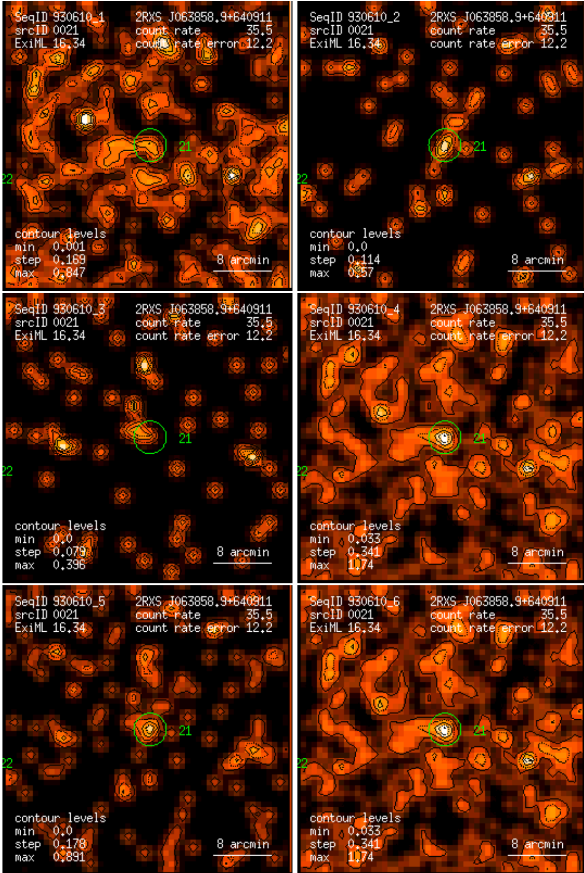
Figure 21: RASS 930610: detection 0021: band rate images, Gaussian filter: (1) PSPC channels 11 – 41, (2) 52 – 90, (3) 91 – 201, (4) 11 – 235, (5) 52 – 201, (6) 11 – 201. Broad band rates in counts/ks. Band rate contour levels in counts/ks/arcmin 2 .
