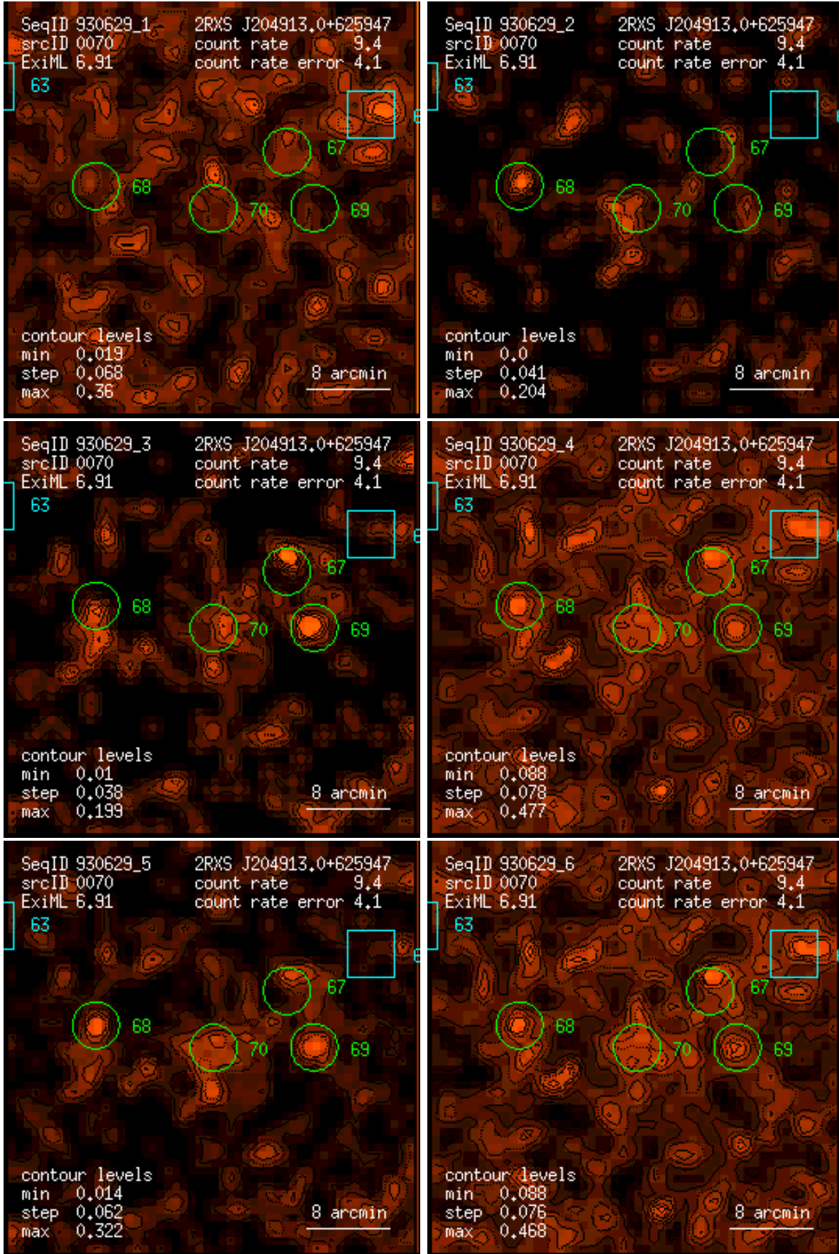
Figure 70: RASS 930629: detection 0070: band rate images, Gaussian filter: (1) PSPC channels 11 – 41, (2) 52 – 90, (3) 91 – 201, (4) 11 – 235, (5) 52 – 201, (6) 11 – 201. Broad band rates in counts/ks. Band rate contour levels in counts/ks/arcmin 2 .
