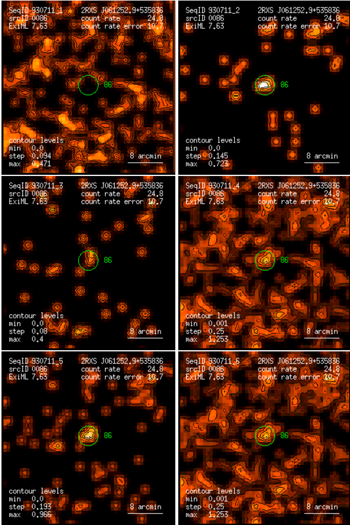
Figure 86: RASS 930711: detection 0086: band rate images, Gaussian filter: (1) PSPC channels 11 – 41, (2) 52 – 90, (3) 91 – 201, (4) 11 – 235, (5) 52 – 201, (6) 11 – 201. Broad band rates in counts/ks. Band rate contour levels in counts/ks/arcmin 2 .
