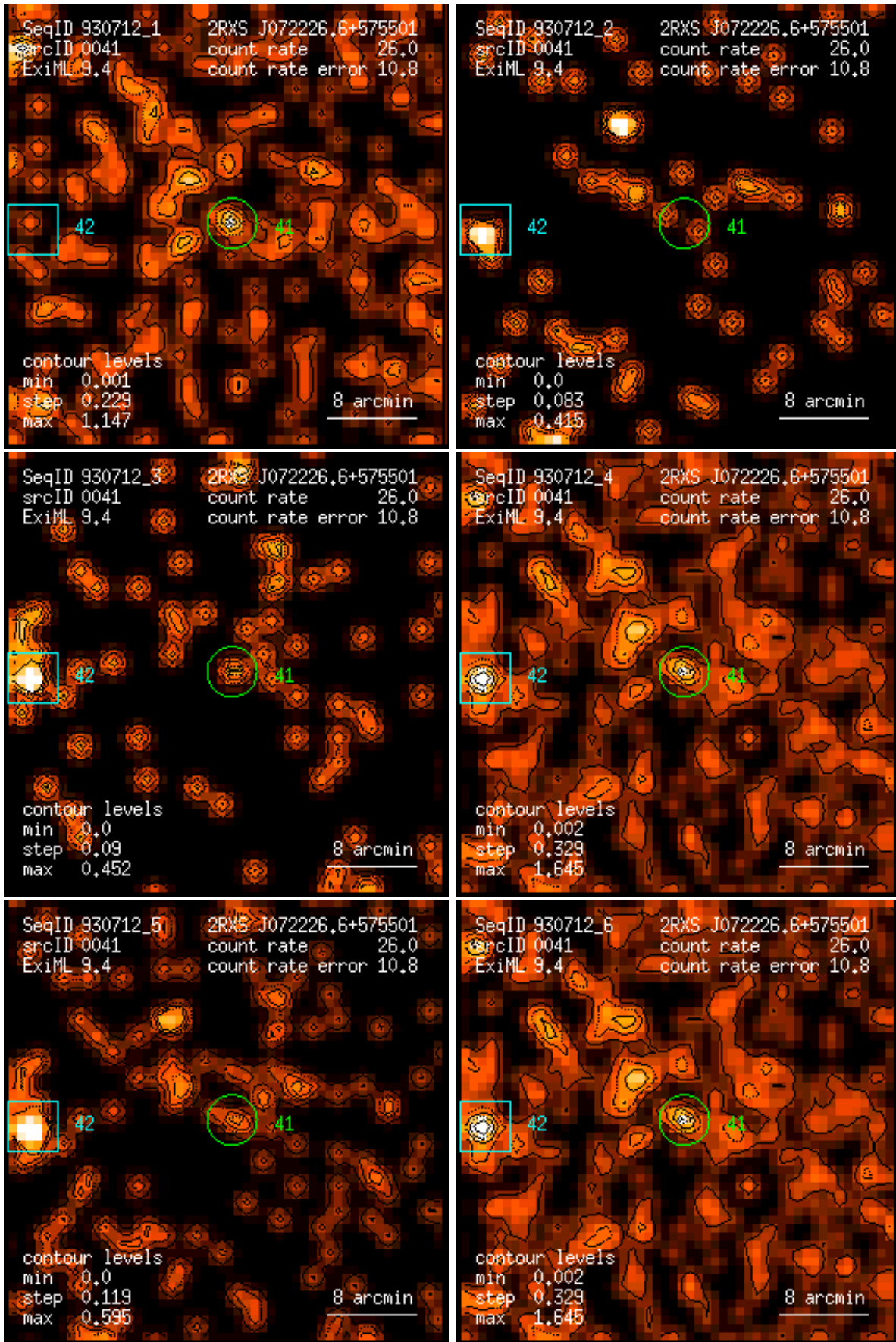
Figure 41: RASS 930712: detection 0041: band rate images, Gaussian filter: (1) PSPC channels 11 – 41, (2) 52 – 90, (3) 91 – 201, (4) 11 – 235, (5) 52 – 201, (6) 11 – 201. Broad band rates in counts/ks. Band rate contour levels in counts/ks/arcmin 2 .
