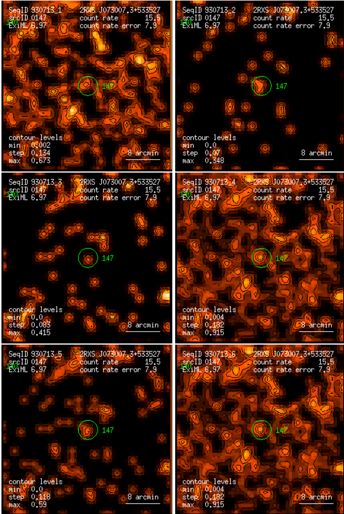
Figure 147: RASS 930713: detection 0147: band rate images, Gaussian filter: (1) PSPC channels 11 – 41, (2) 52 – 90, (3) 91 – 201, (4) 11 – 235, (5) 52 – 201, (6) 11 – 201. Broad band rates in counts/ks. Band rate contour levels in counts/ks/arcmin 2 .
