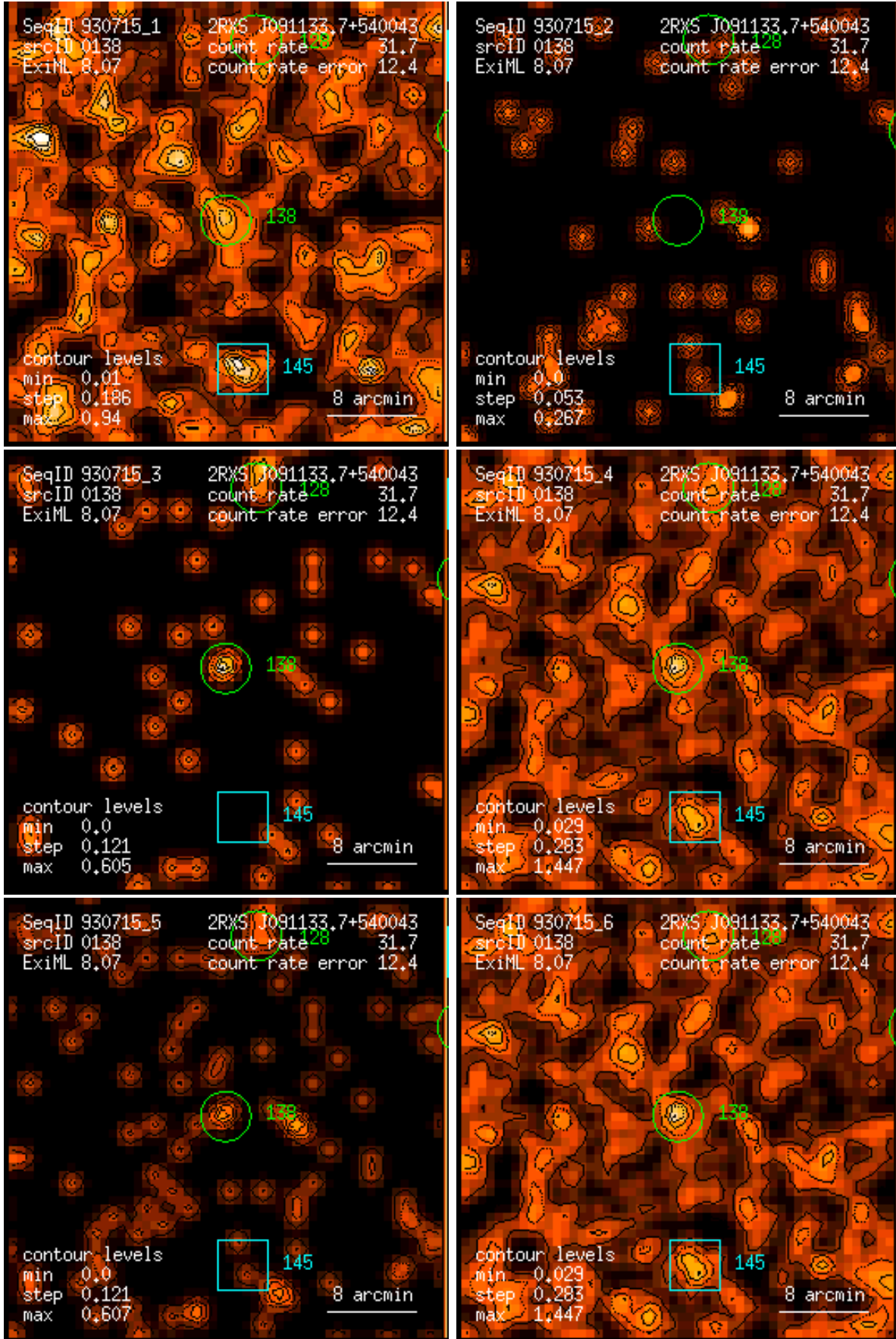
Figure 138: RASS 930715: detection 0138: band rate images, Gaussian filter: (1) PSPC channels 11 – 41, (2) 52 – 90, (3) 91 – 201, (4) 11 – 235, (5) 52 – 201, (6) 11 – 201. Broad band rates in counts/ks. Band rate contour levels in counts/ks/arcmin 2 .
