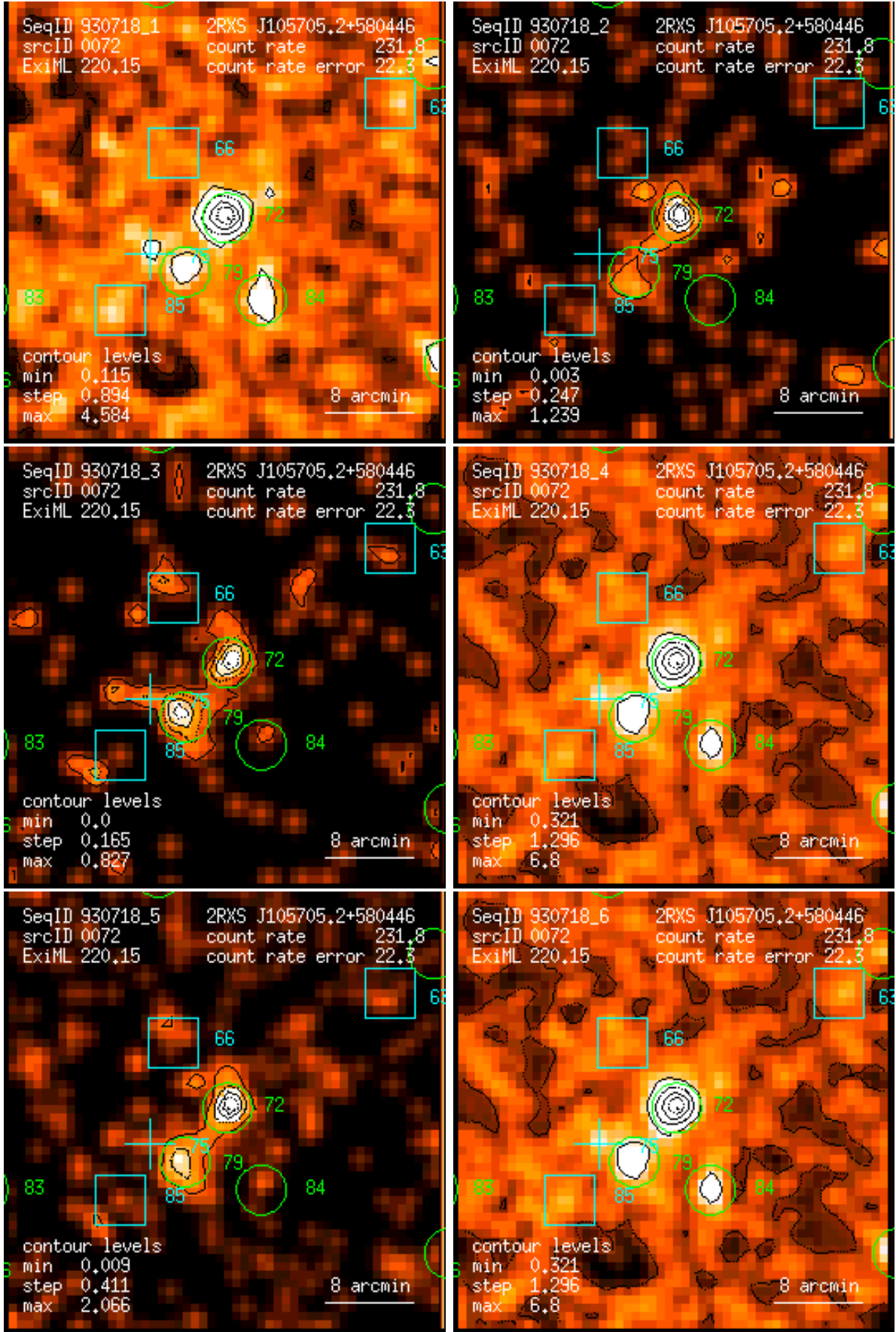
Figure 72: RASS 930718: detection 0072: band rate images, Gaussian filter: (1) PSPC channels 11 – 41, (2) 52 – 90, (3) 91 – 201, (4) 11 – 235, (5) 52 – 201, (6) 11 – 201. Broad band rates in counts/ks. Band rate contour levels in counts/ks/arcmin 2 .
