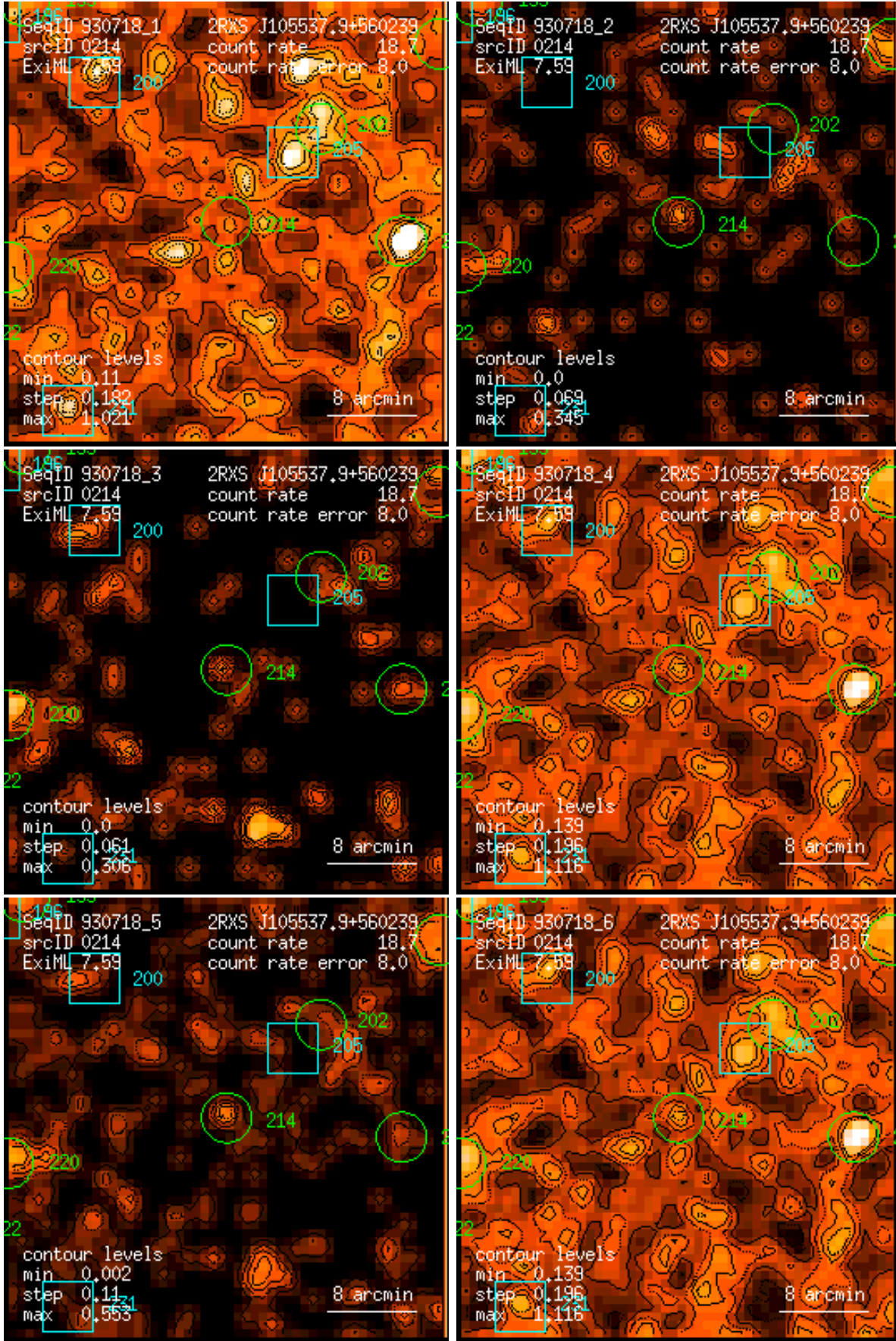
Figure 214: RASS 930718: detection 0214: band rate images, Gaussian filter: (1) PSPC channels 11 – 41, (2) 52 – 90, (3) 91 – 201, (4) 11 – 235, (5) 52 – 201, (6) 11 – 201. Broad band rates in counts/ks. Band rate contour levels in counts/ks/arcmin 2 .
