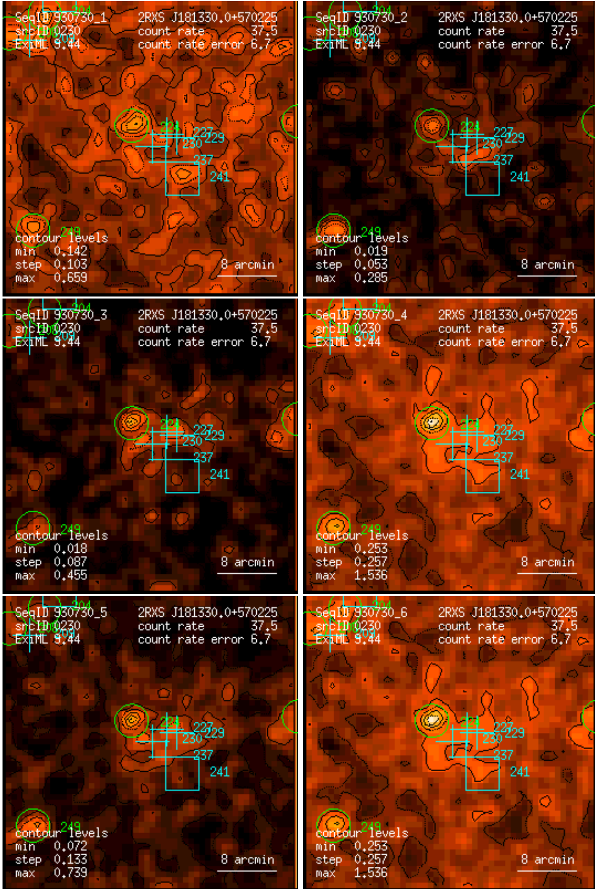
Figure 230: RASS 930730: detection 0230: band rate images, Gaussian filter: (1) PSPC channels 11 – 41, (2) 52 – 90, (3) 91 – 201, (4) 11 – 235, (5) 52 – 201, (6) 11 – 201. Broad band rates in counts/ks. Band rate contour levels in counts/ks/arcmin 2 .
