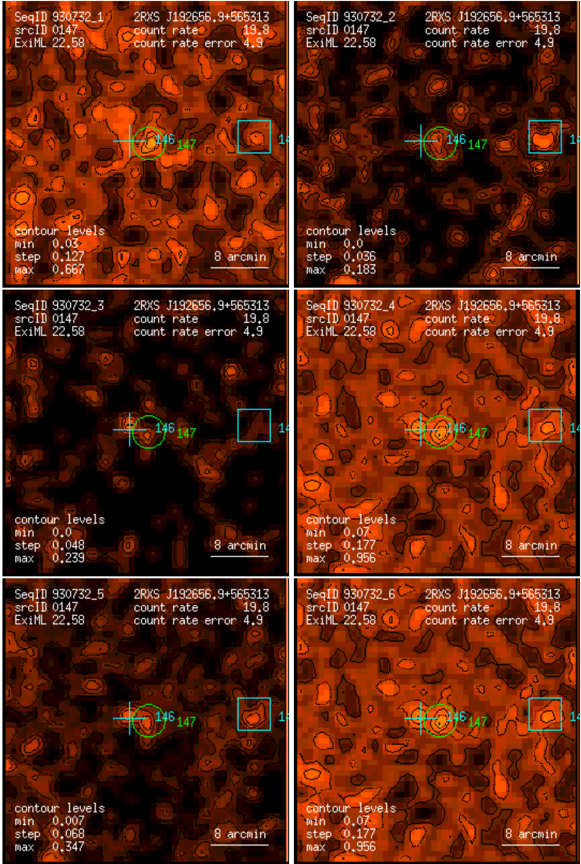
Figure 147: RASS 930732: detection 0147: band rate images, Gaussian filter: (1) PSPC channels 11 – 41, (2) 52 – 90, (3) 91 – 201, (4) 11 – 235, (5) 52 – 201, (6) 11 – 201. Broad band rates in counts/ks. Band rate contour levels in counts/ks/arcmin 2 .
