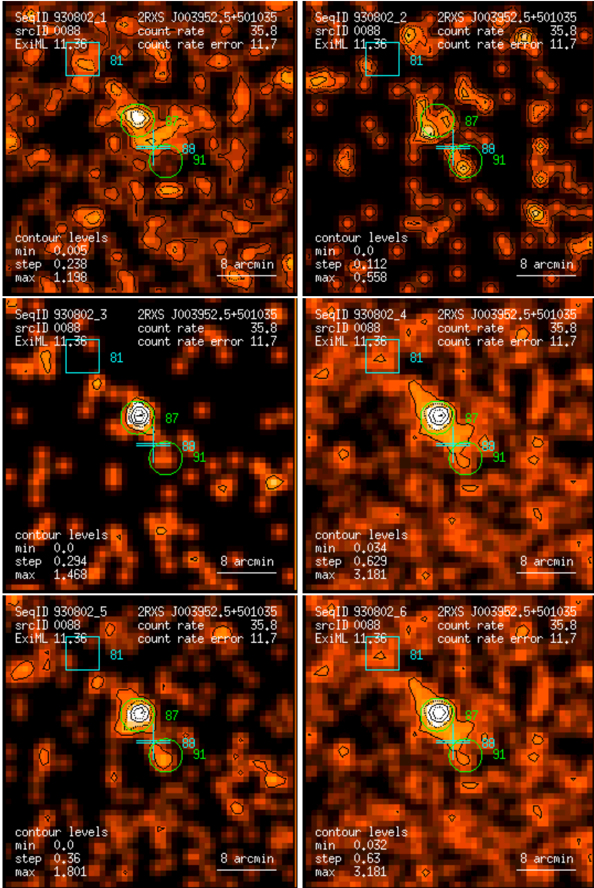
Figure 88: RASS 930802: detection 0088: band rate images, Gaussian filter: (1) PSPC channels 11 – 41, (2) 52 – 90, (3) 91 – 201, (4) 11 – 235, (5) 52 – 201, (6) 11 – 201. Broad band rates in counts/ks. Band rate contour levels in counts/ks/arcmin 2 .
