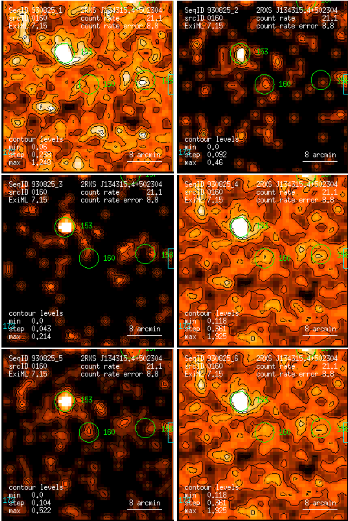
Figure 160: RASS 930825: detection 0160: band rate images, Gaussian filter: (1) PSPC channels 11 – 41, (2) 52 – 90, (3) 91 – 201, (4) 11 – 235, (5) 52 – 201, (6) 11 – 201. Broad band rates in counts/ks. Band rate contour levels in counts/ks/arcmin 2 .
